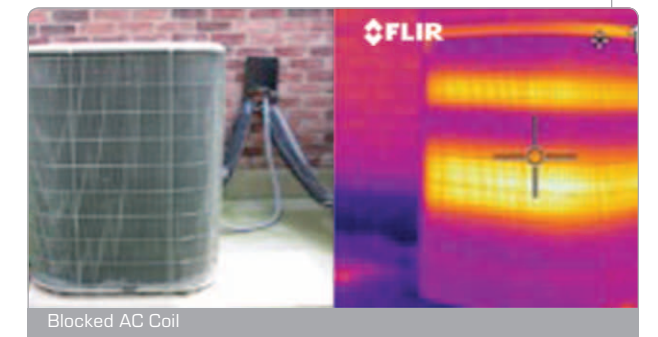
Blocked AC Coil
