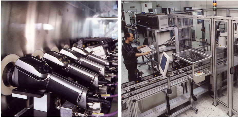
Figure 15.4 LEFT: Testing of infrared cameras in the climatic chamber; RIGHT: Robot used for camera testing and calibration
