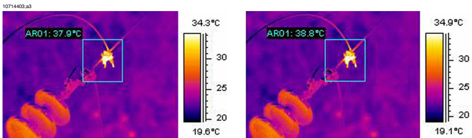
Figure 14.18 LEFT: Incorrect distance setting; RIGHT: Correct distance setting
