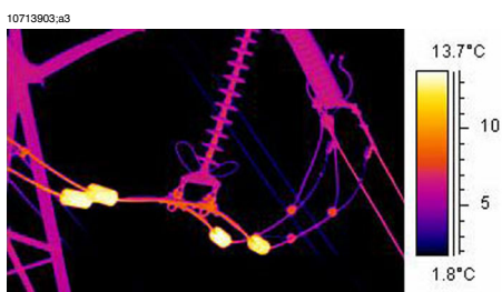
Figure 14.13 An infrared image of hot stabilizing weights
