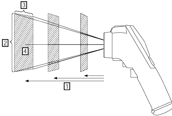
Figure 11.1 Relationship between field of view and distance. 1: Distance to target; 2: VFOV = vertical field of view; 3: HFOV = horizontal field of view; 4: IFOV = instantaneous field of view (size of one detector element).
