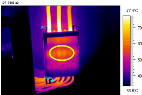
Figure 14.4 A hidden hot spot inside a box
