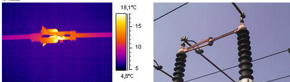
Figure 14.17 Overheating in a circuit breaker
