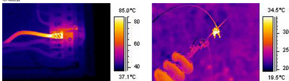
Figure 14.16 LEFT: An infrared image showing bad contact due to a loose bolt; RIGHT: A loose outdoor connection, exposed to the wind cooling effect.
