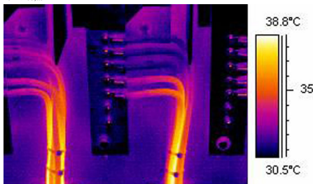
Figure 14.15 An infrared image of bundled cables
