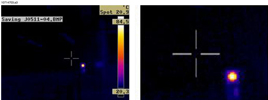
Figure 14.21 Image from the viewfinder of a ThermoCAM 695
