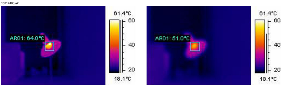
Figure 14.5 LEFT: A hot spot in focus; RIGHT: A hot spot out of focus
