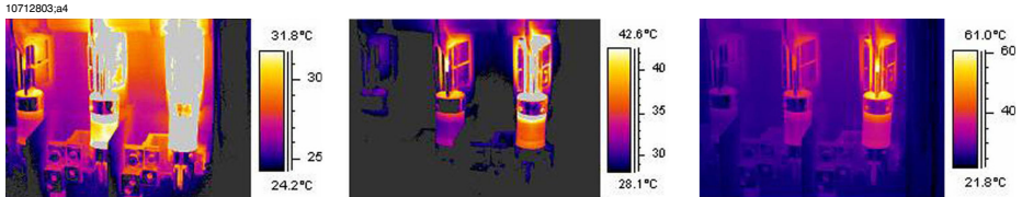
Figure 14.2 Temperature variations in a fusebox
