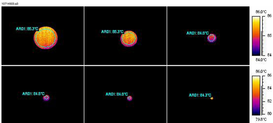
Figure 14.19 Temperature readings from a blackbody at +85°C (+185°F) at increasing distances
