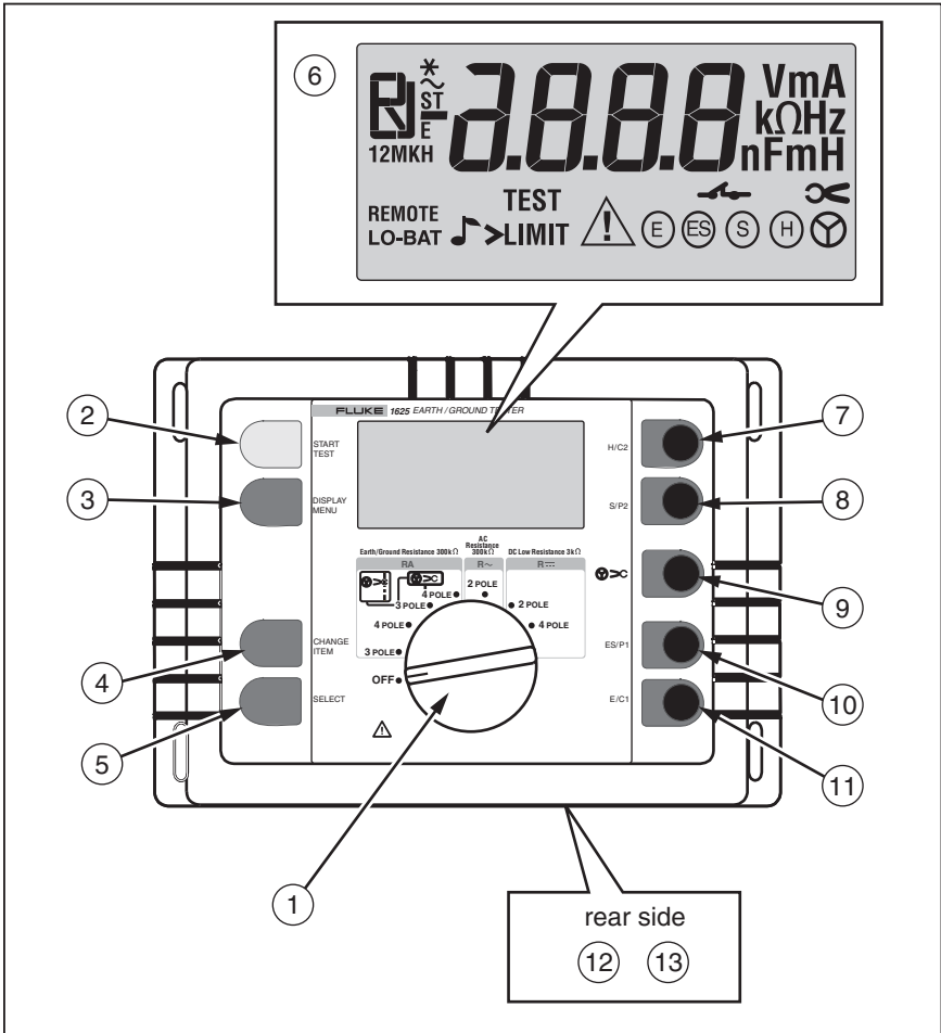
Figure 2. Operating Elements
