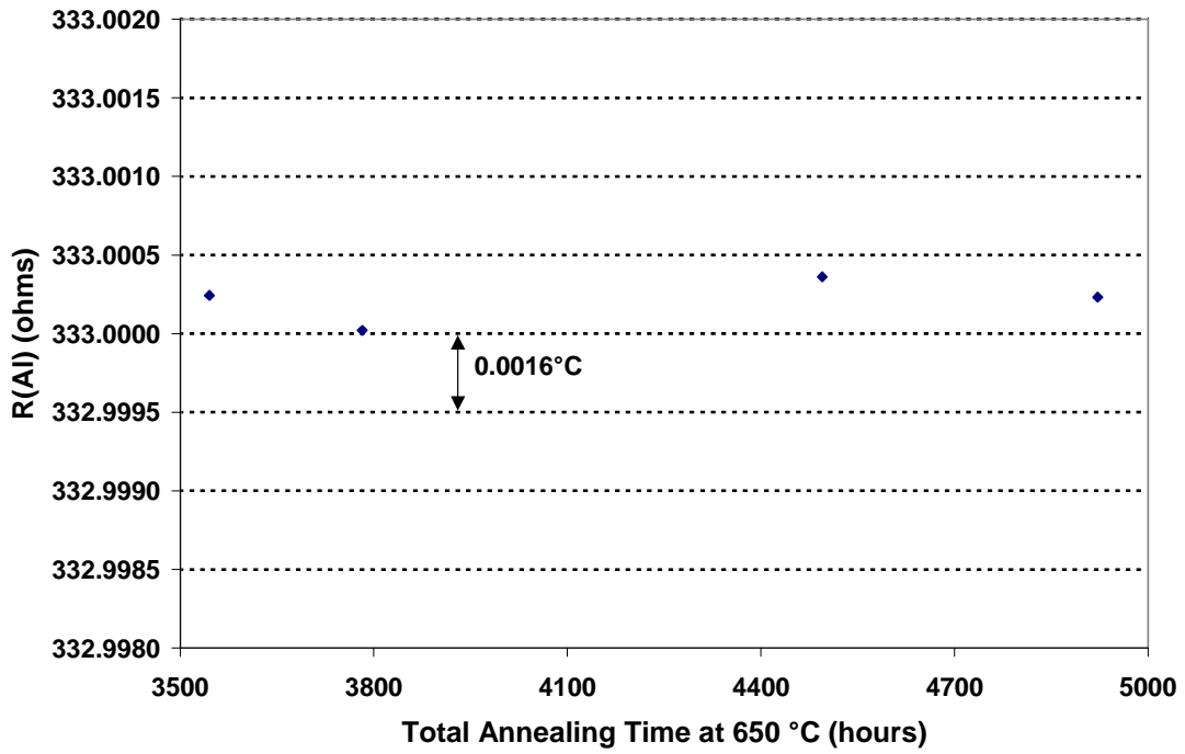
Fig. 9. The resistance R(Al) of K-1 during annealing at 650°C
