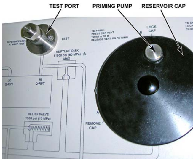
Figure 1: E-DWT top view
