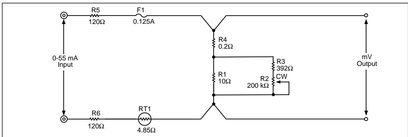
Schematic Diagram
