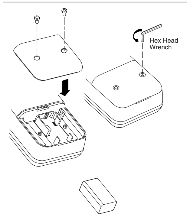
Figure 7. Battery Replacement
