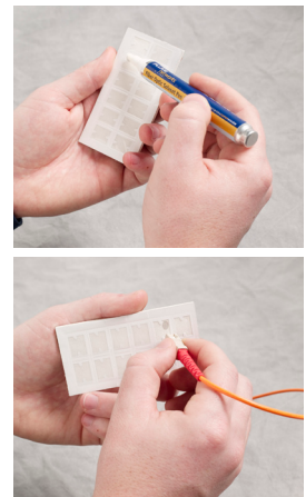
The right tools will help with fiber end face cleaning. Solvent from a fiber optic solvent pen, applied to a special purpose, disposable cleaning pad, is a best-practice method cleaning fiber optic cabling.
