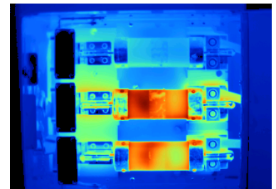
Three-phase switchgear load imbalance or single-phasing.
