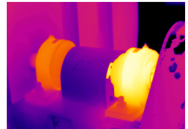
Overheating bearing cap.
