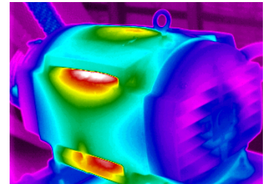
Abnormal or uneven heating on motor.
