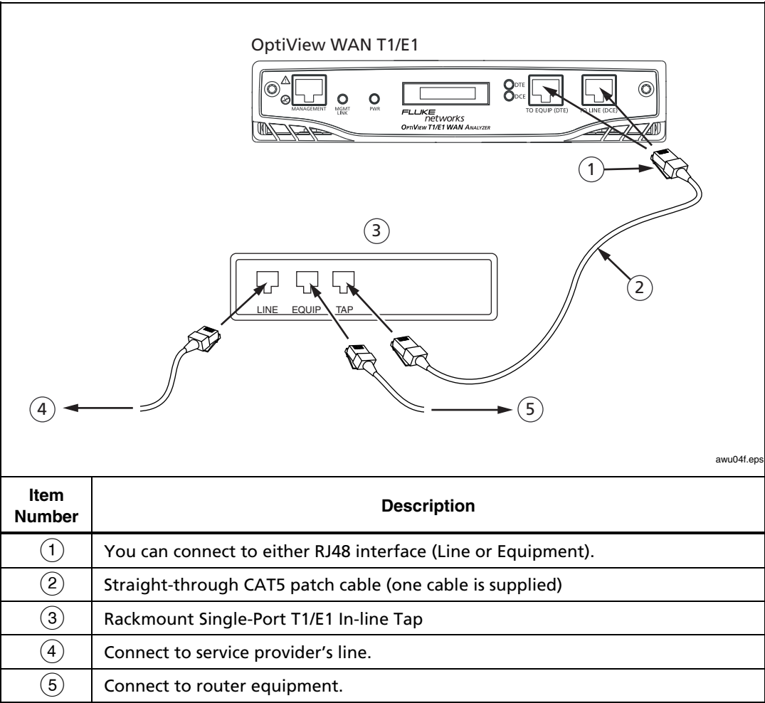
Figure 4. Connecting to a Rackmount Single Port T1/E1 In-Line Tap
