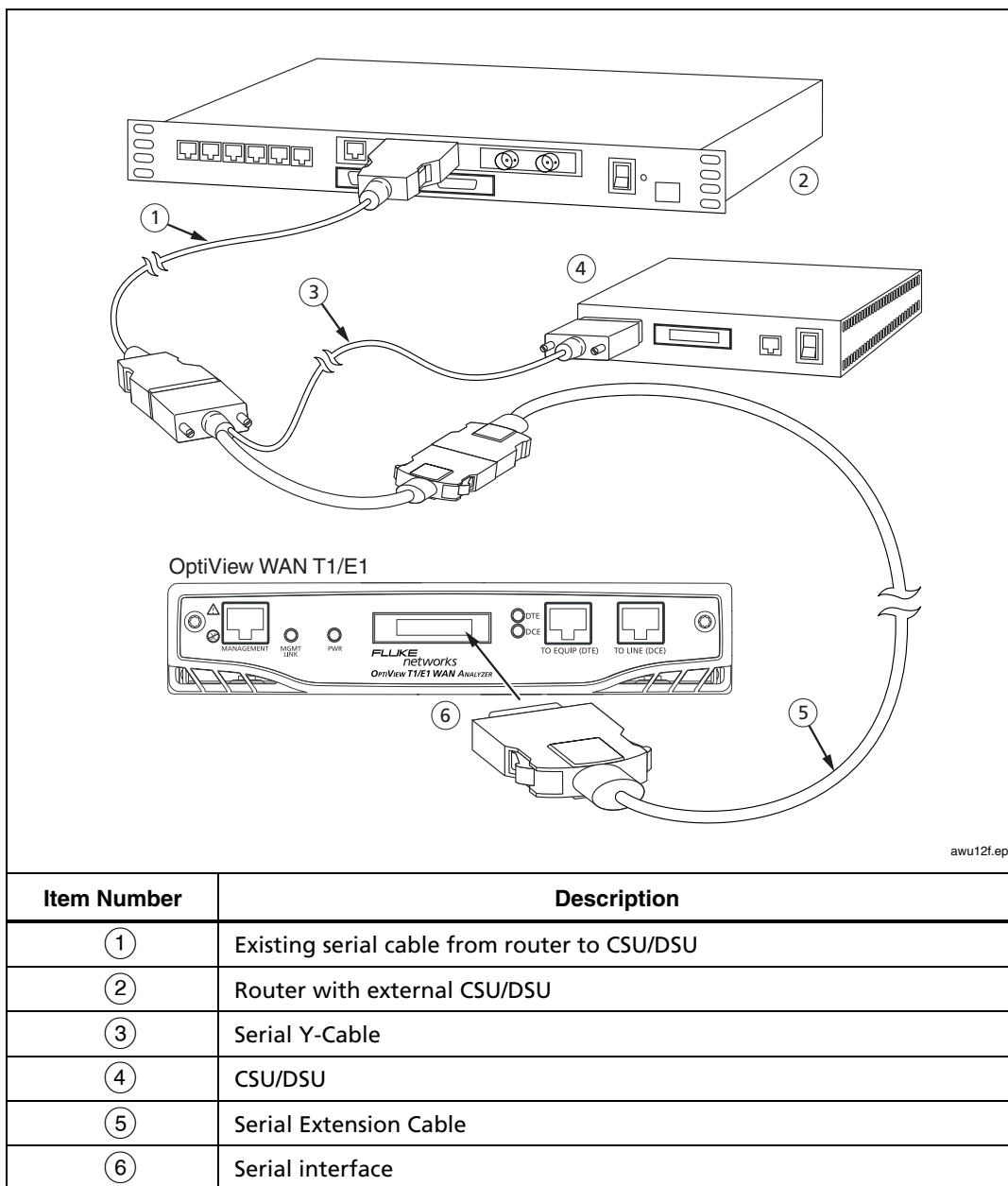
Figure 6. T1/E1 Tap with Serial Y-Cable Access
