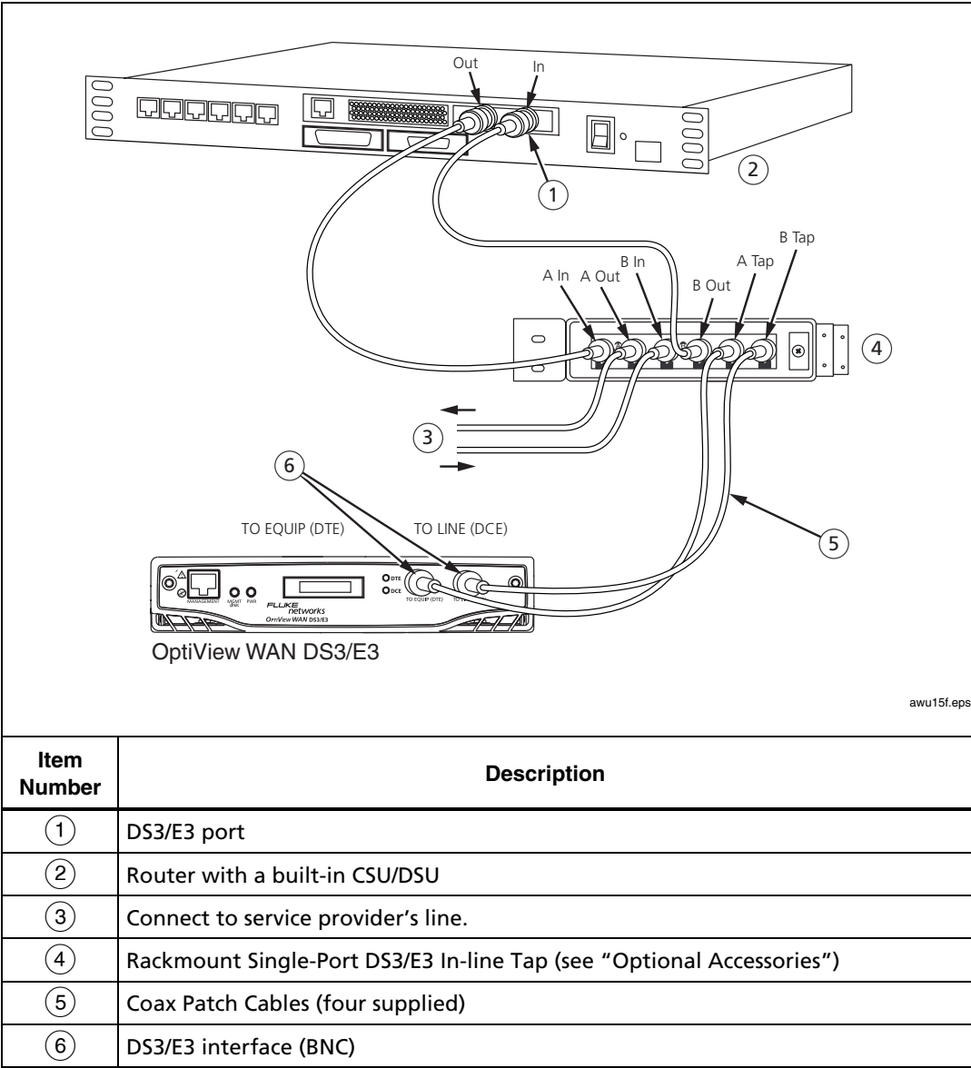
Figure 8. Connecting to a Rackmount Single-Port DS3/E3 In-Line Tap
