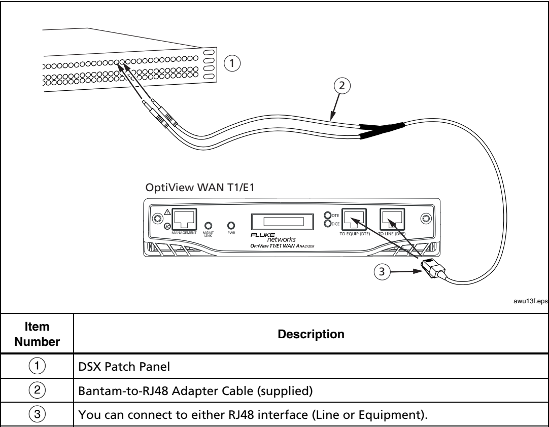
Figure 7. Connecting to the T1/E1 Monitor Jacks on a DSX Patch Panel
