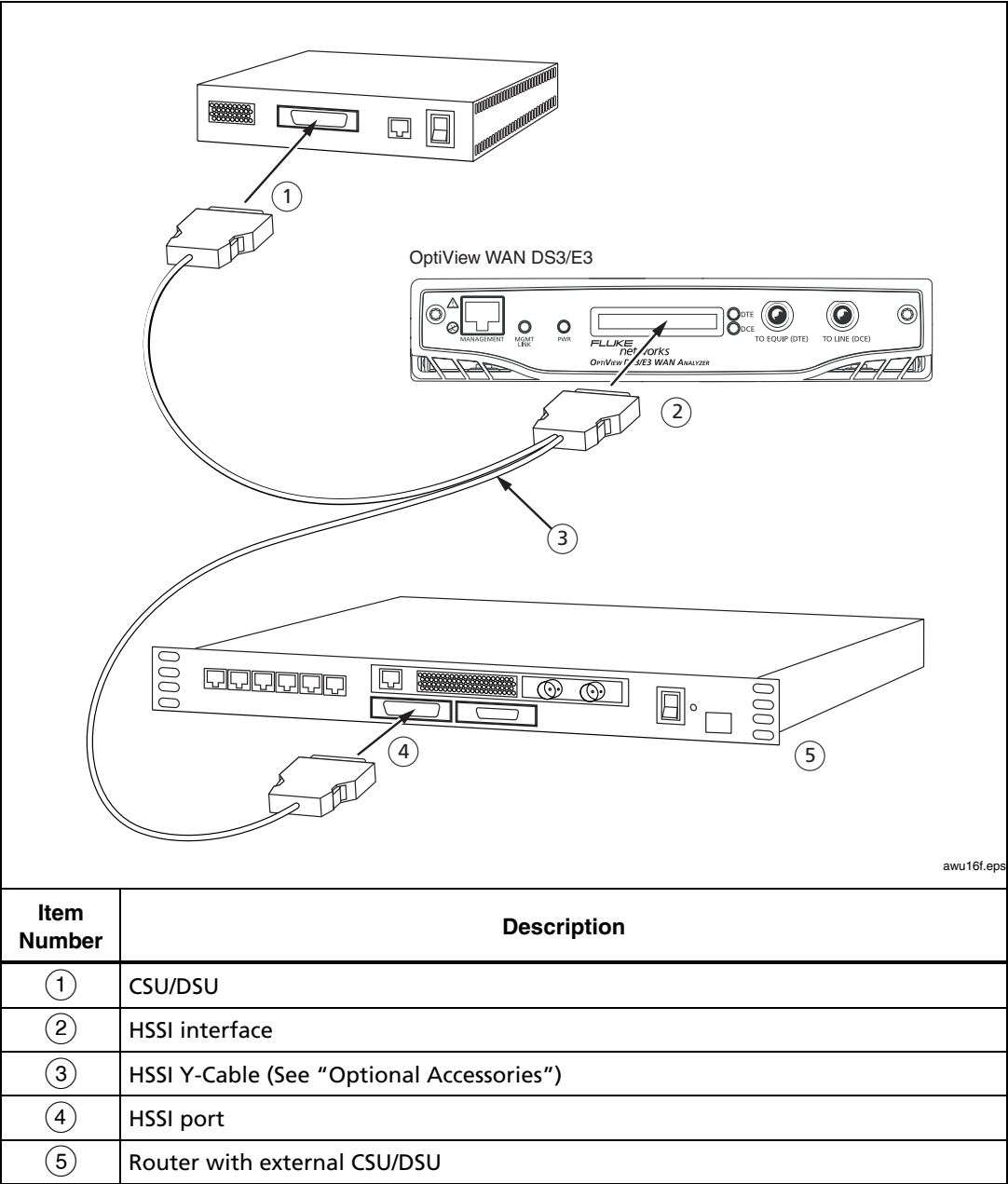
Figure 9. DS3/E3 Tap with HSSI Y-Cable Access
