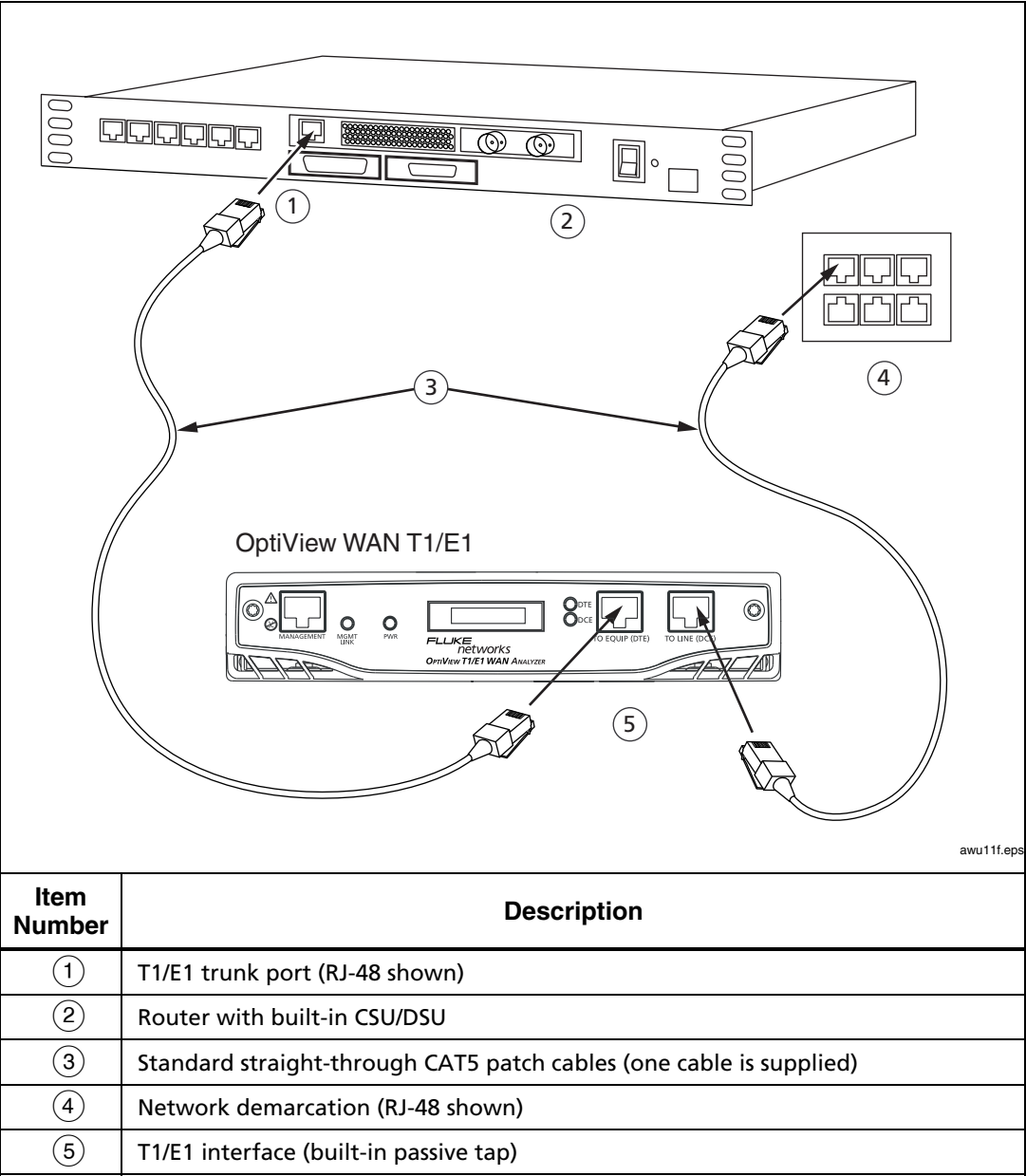
Figure 5. Connecting to the Network Using the Built-In Tap
