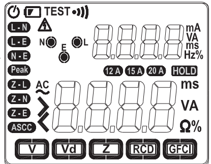
Fig. 2. All possible indications on the CA10's LCD
