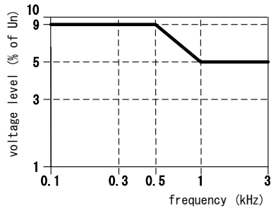
Mains signaling voltage on the supply voltage threshold default value
