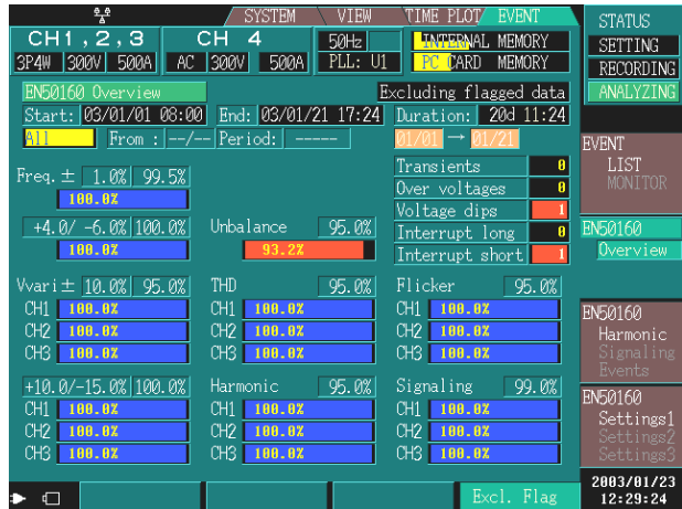
EN50160 Overview Screen
