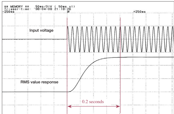
Analog output response of the 3331/3332
