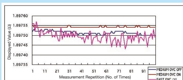
[ Low-Power Ohms: 2 W Range/FAST & MEDIUM ]
