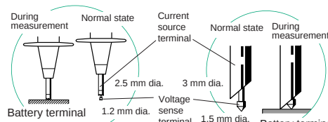
9465 PIN TYPE LEADS -- detail 9461 PIN TYPE LEADS -- detail
