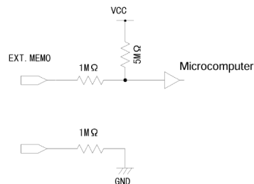
Circuit configuration of EXT.MEMO in 3550
