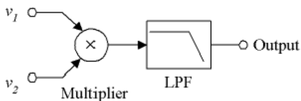
Fig. 3: Synchronous detection circuit
