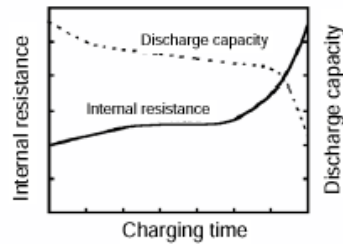
Correlation between charging time and internal resistance
