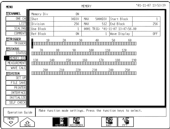
Memory segmentation screen (MEMORY DIV)
