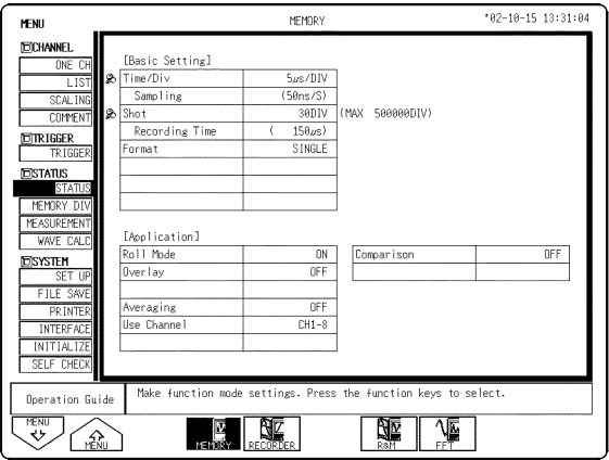
Status screen
