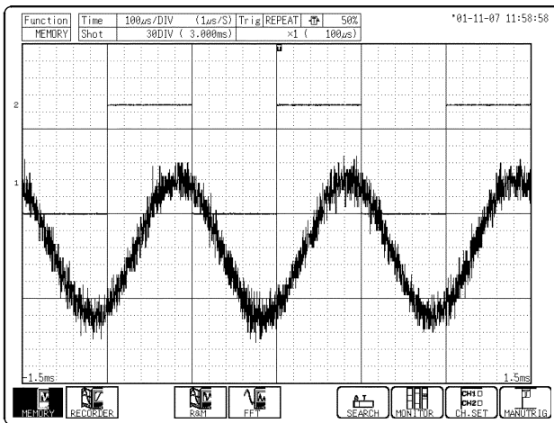
Before Averaging
