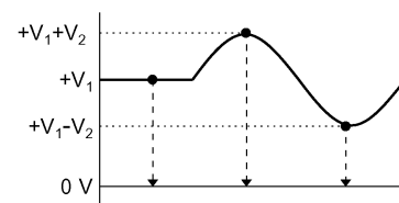
When input voltage is fluctuating
