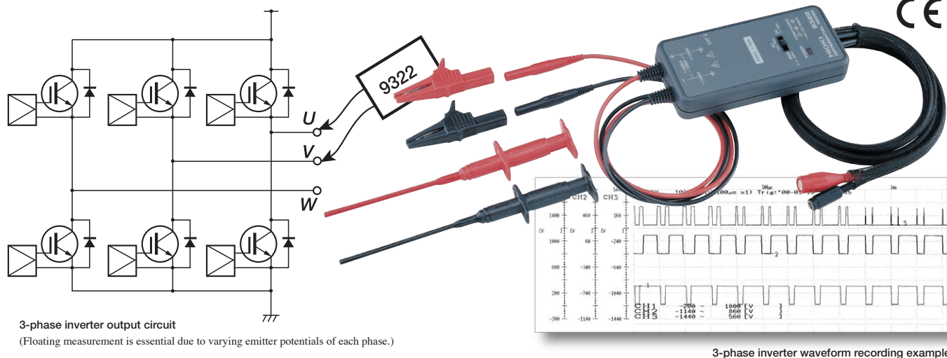
3-phase inverter waveform recording example
