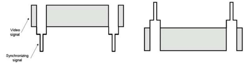
Figure 5-13(a) (▭▭) Sync signal
