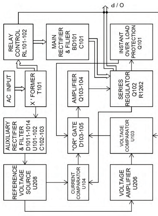
Block diagram
