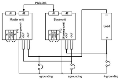
Series Connection
