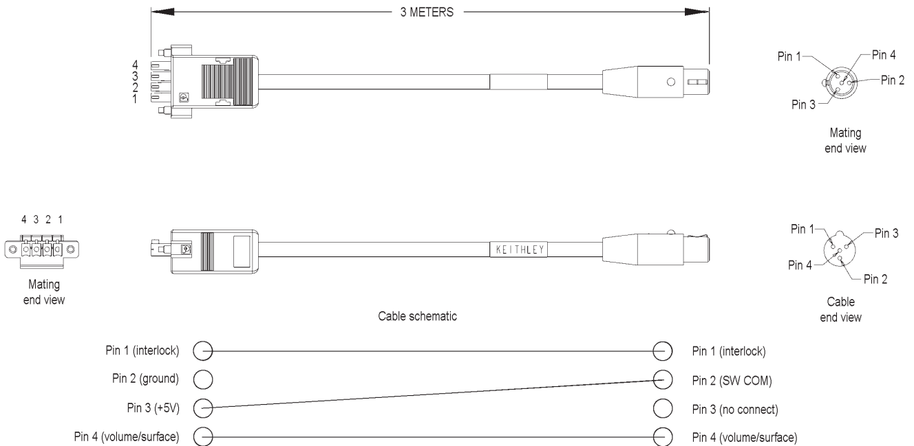
Figure 1 6517B-ILC-3 Interlock Cable
