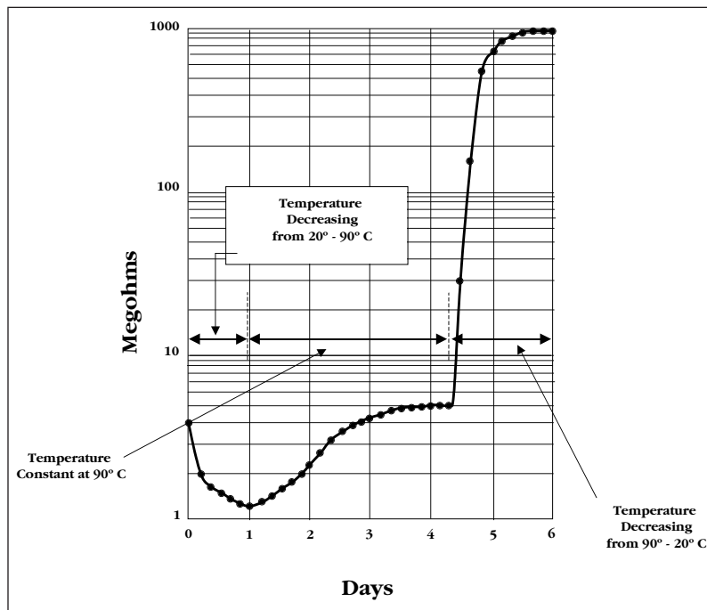
Figure 22: Typical Drying-out Resistance Graph
