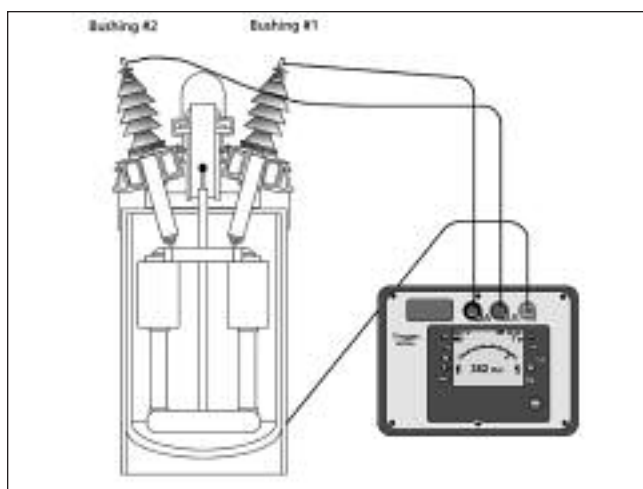
Figure 5: Connection to a Circuit Breaker
