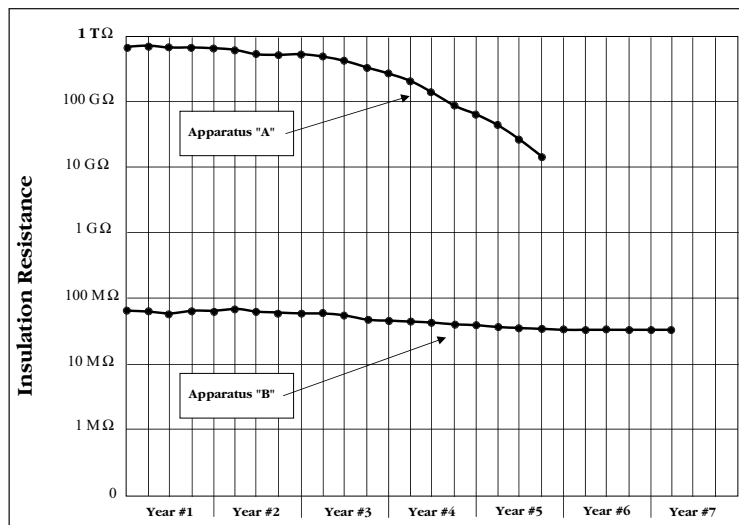
Figure 12: Comparison of Trended Test Results
