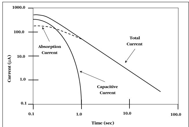
Figure 17: Reabsorption Currents
