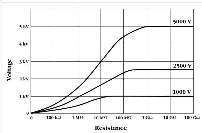
Figure 10: Poor Load Curve
