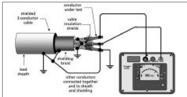
Figure 4: Connection to a Shielded Power Cable
