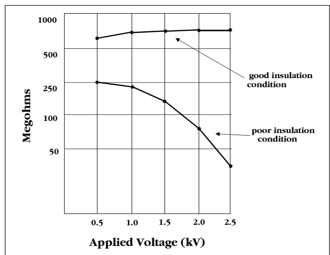
Figure 15: Step Voltage Step Graph
