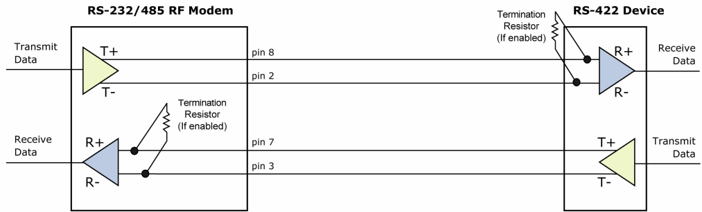
Figure 2.14. AWB-S RF Modem in an RS-485 (4-wire) environment
