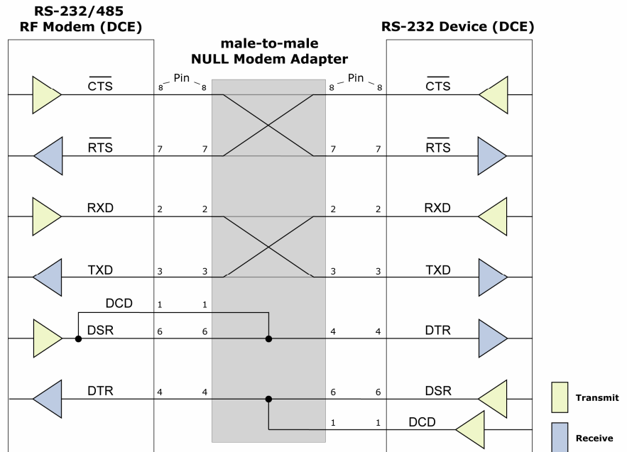
Figure 2.4. AWB-S RF Modem (female connector) wired to an RS-232 DTE (male connector) device
