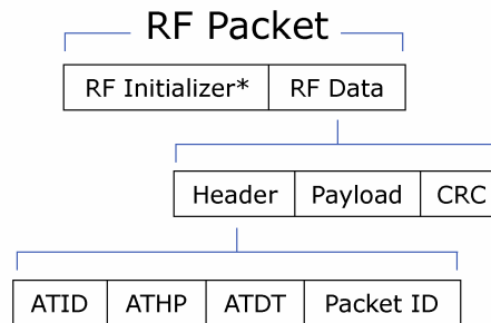
Figure 3.5. RF Packet Components
