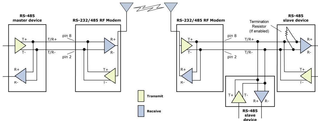
Figure 2.9. AWB-S RF Modem in an RS-485 (2-wire) half-duplex environment
