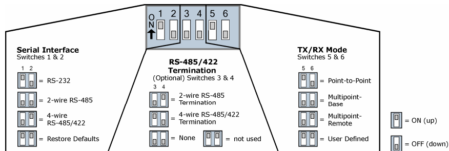
Figure 1.3. DIP Switch Settings
