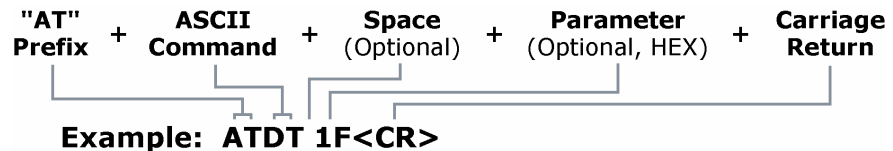
Figure 3.8. Syntax for sending AWB-S AT Commands
