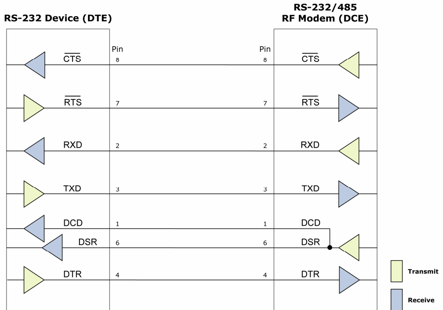
Figure 2.3. RS-232 DTE (male connector) device wired to an AWB-S RF Modem (female connector)
