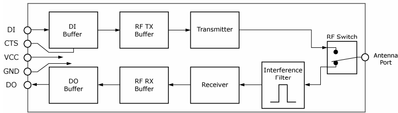
Figure 3.2. Internal Data Flow Diagram
