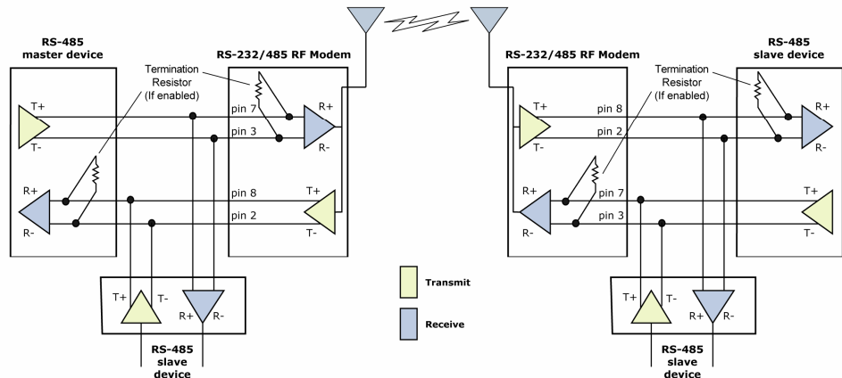
Figure 2.13. AWB-S RF Modem in an RS-485 (4-wire) environment
