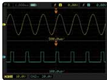
Alternative Trigger
