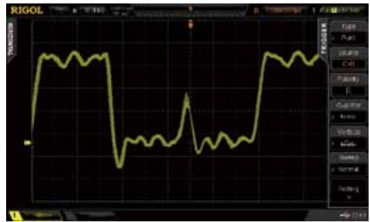
Runt Trigger
