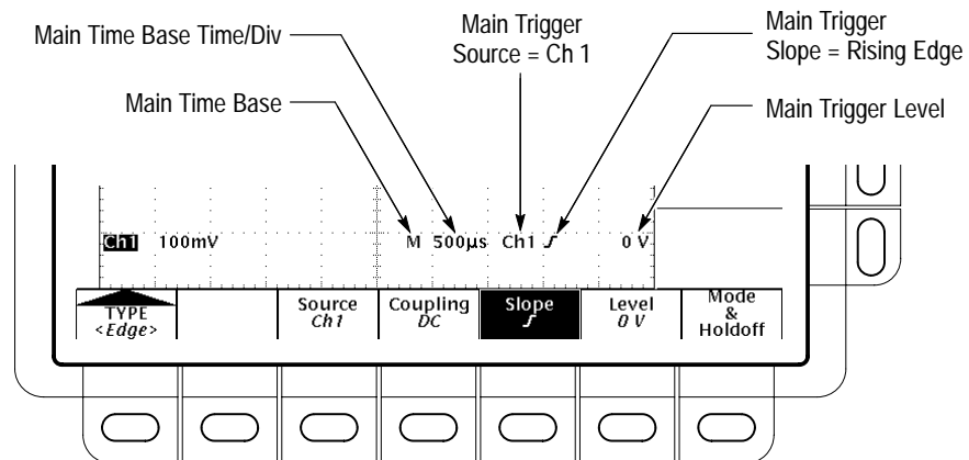
Figure 3–11: Edge Trigger Readouts
