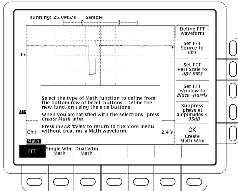
Figure 3–16: Define FFT Waveform Menu
