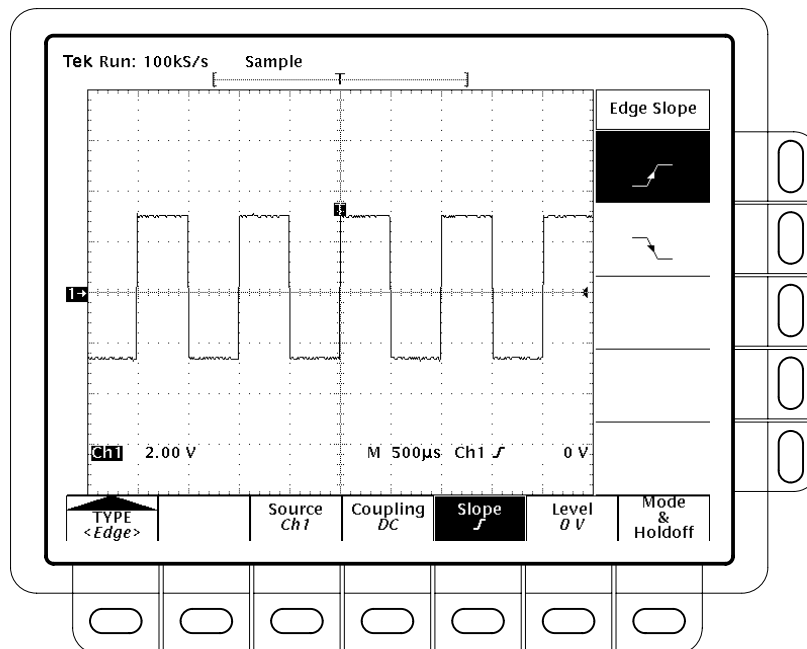
Figure 3-13: Main Trigger Menu — Edge Type
