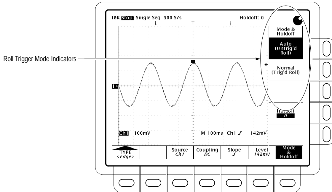
Figure 3-54: Trigger Mode Menu
