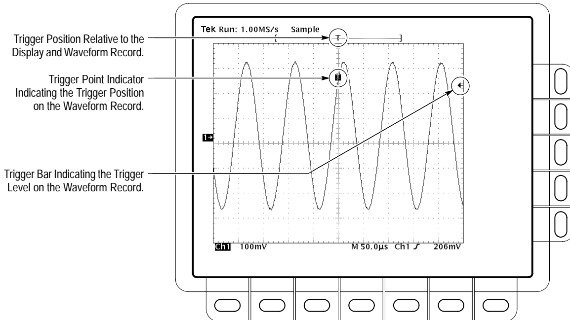
Figure 3–12: Record View, Trigger Position, and Trigger Level Bar Readouts
