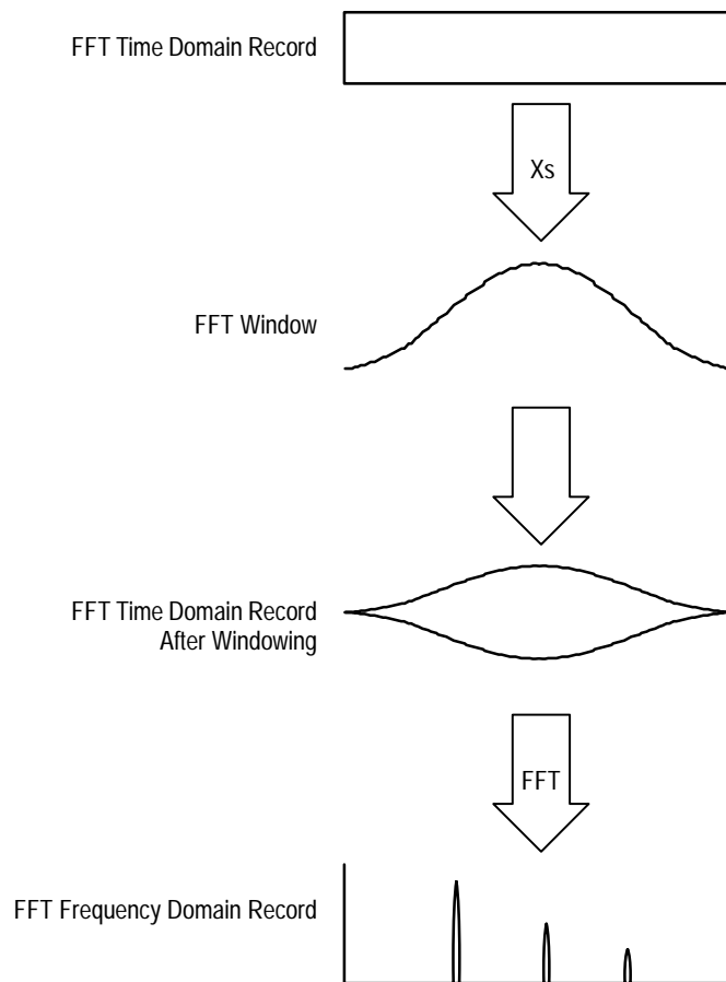
Figure 3–22: Windowing the FFT Time Domain Record
