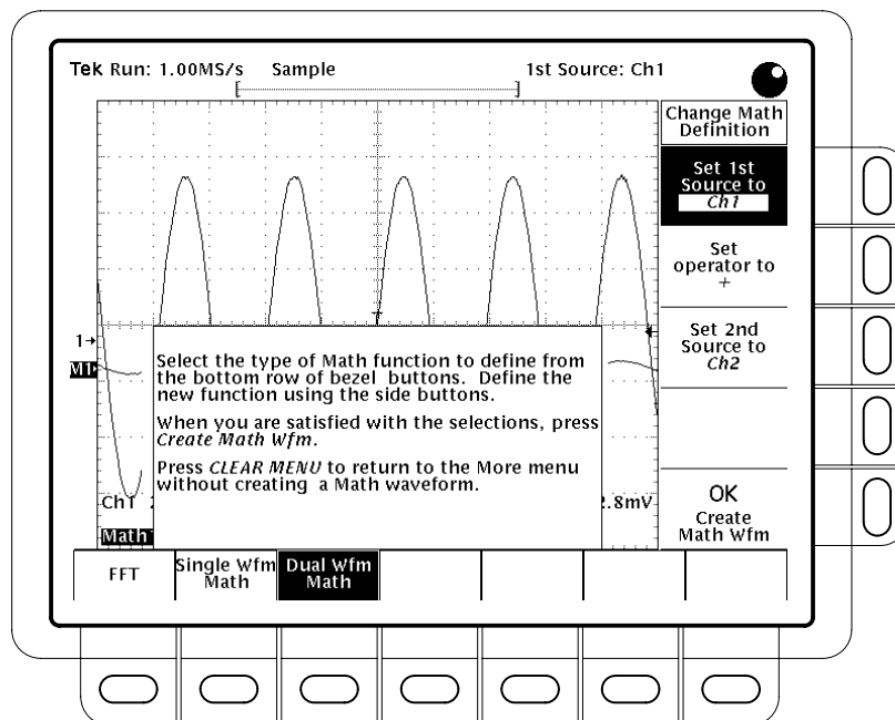
Figure 3–78: Dual Waveform Math Menus
