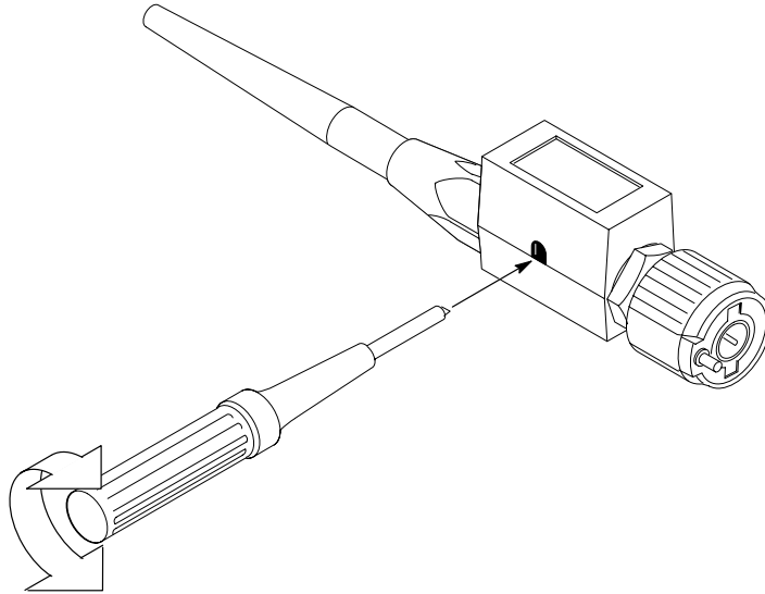
Figure 3-47: Probe Adjustment
