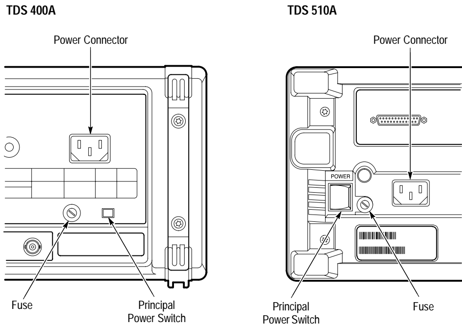
Figure 1-1: Rear Panel Controls Used in Start Up
