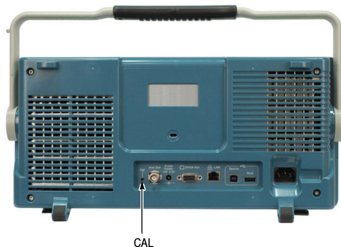
Figure 3-1: Rear panel
