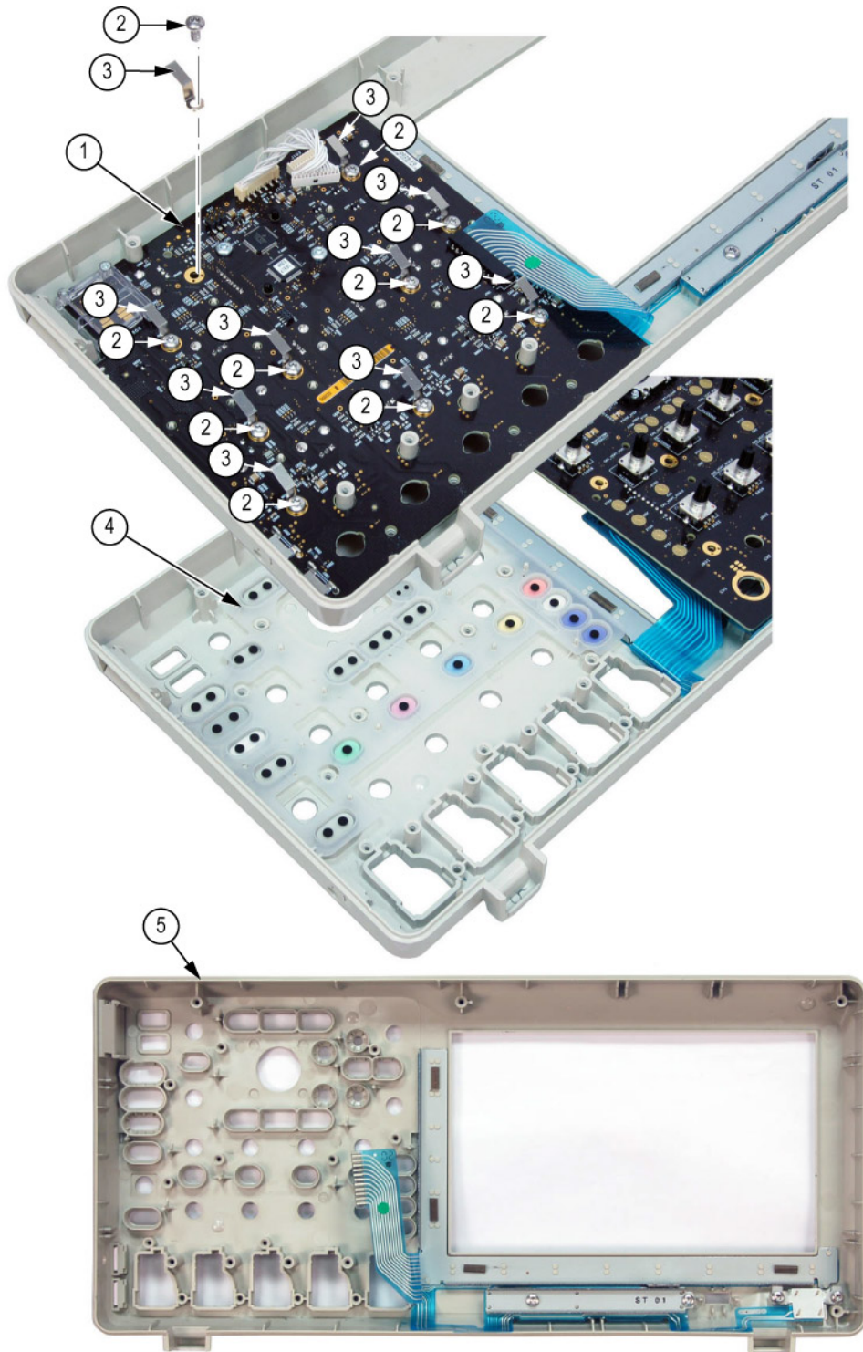
Figure 5-7: Exploded view: DPO3000 front panel board and front case
