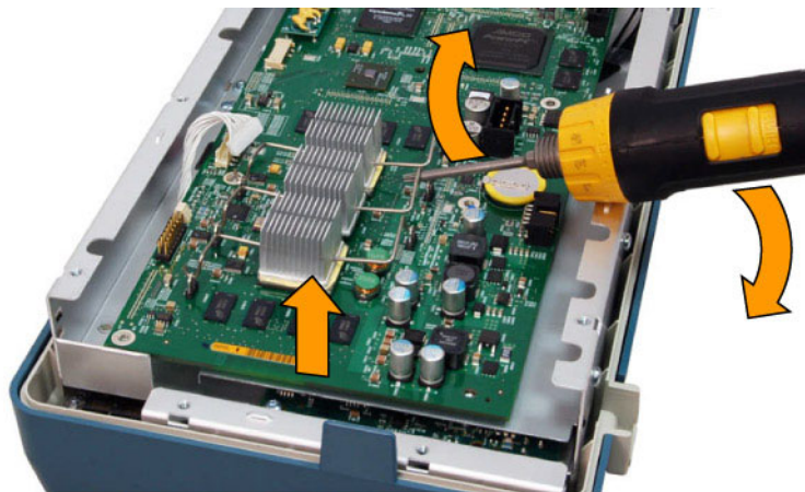
Figure 4-4: Disconnecting the Main board
