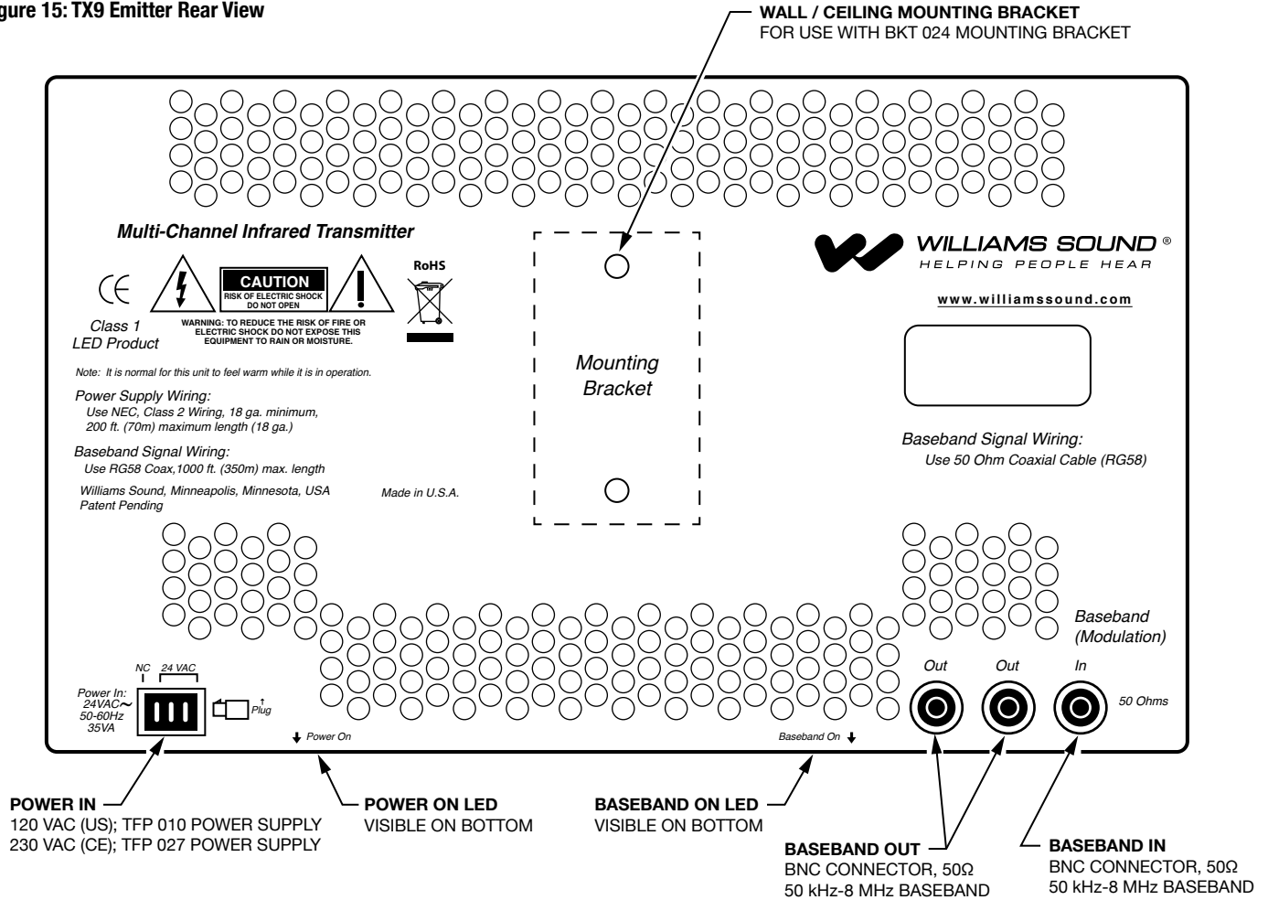
Figure 15: TX9 Emitter Rear View
