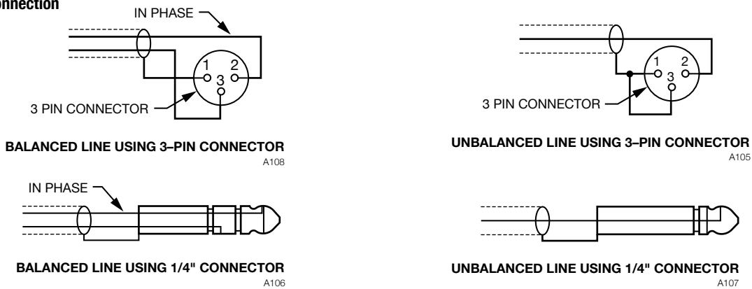
Figure 5: Audio Connection
