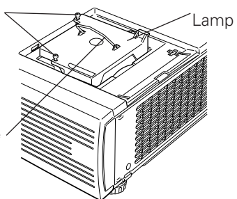
Handle
