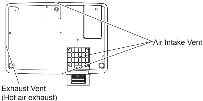
Exhaust Vent (Hot air exhaust)
