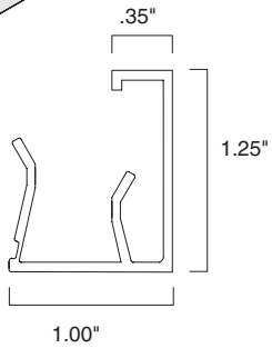
Trim Cross-section
