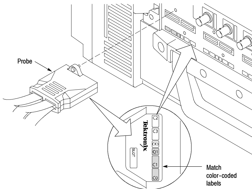
Figure 5: Connecting the probes to the logic analyzer
