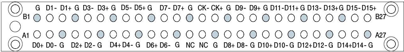
Figure 26: P6980 differential PCB footprint pinout detail
