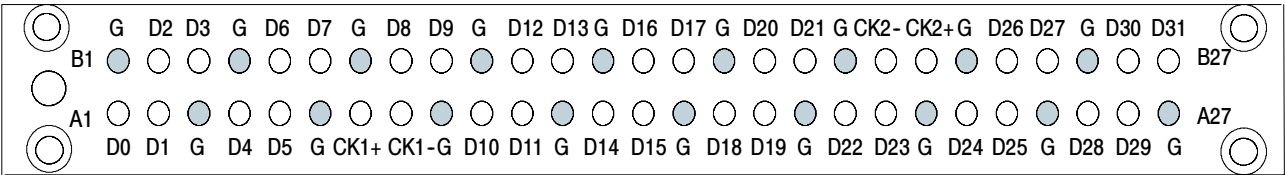
Figure 24: P6960 single-ended PCB footprint pinout detail
