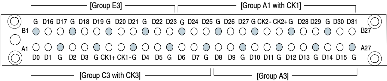
Figure 25: P6964 single-ended PCB footprint pinout detail
