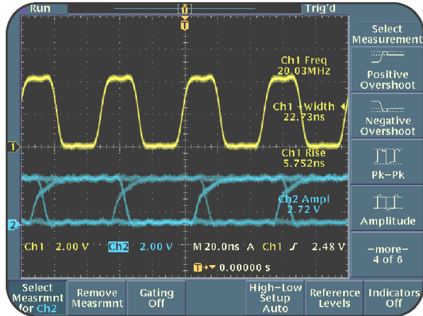
Figure 6.4: Simultaneous amplitude measurement of CH1 and CH2
