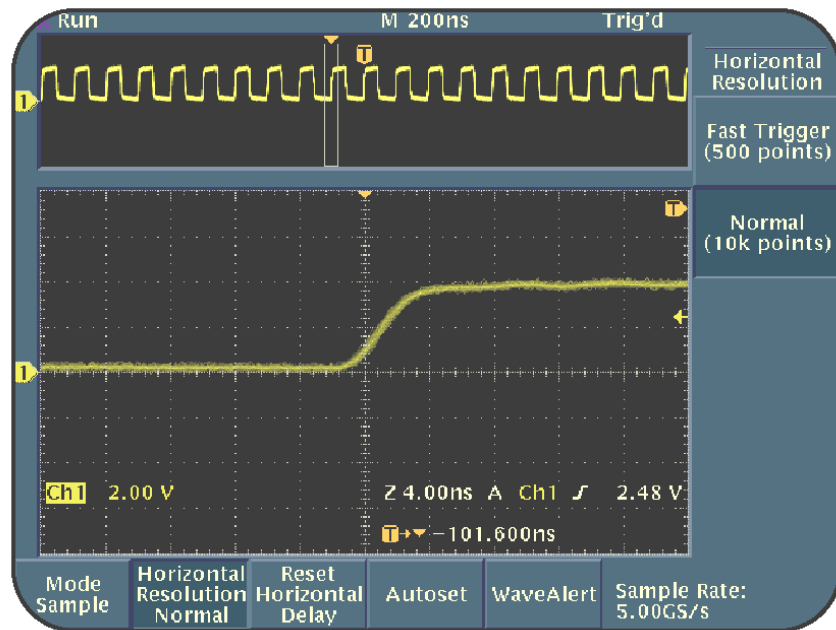
Figure 3.4: Magnified waveform display
