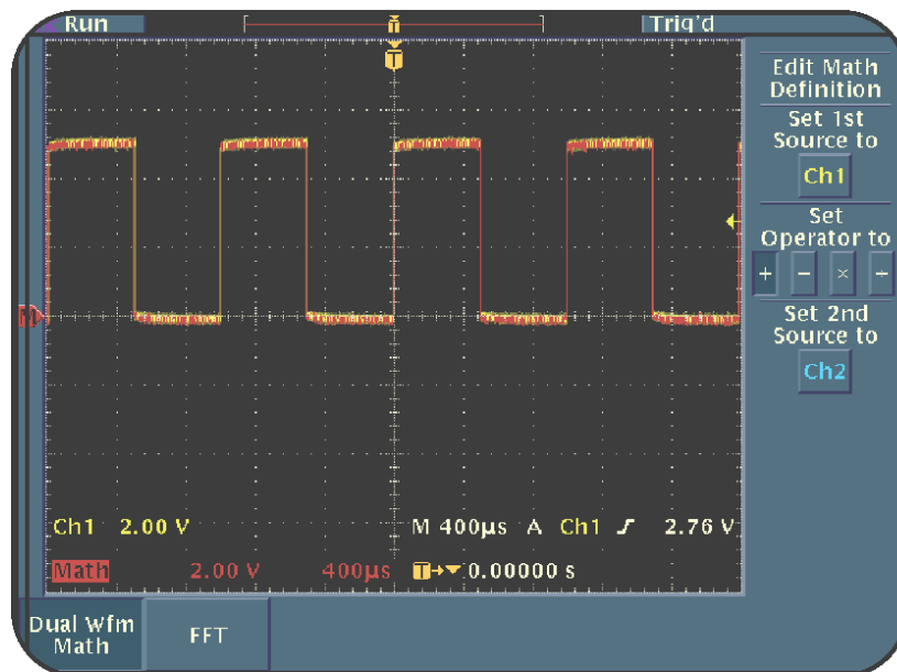
Figure 1.5: TDS3000 oscilloscope MATH menu-based controls
