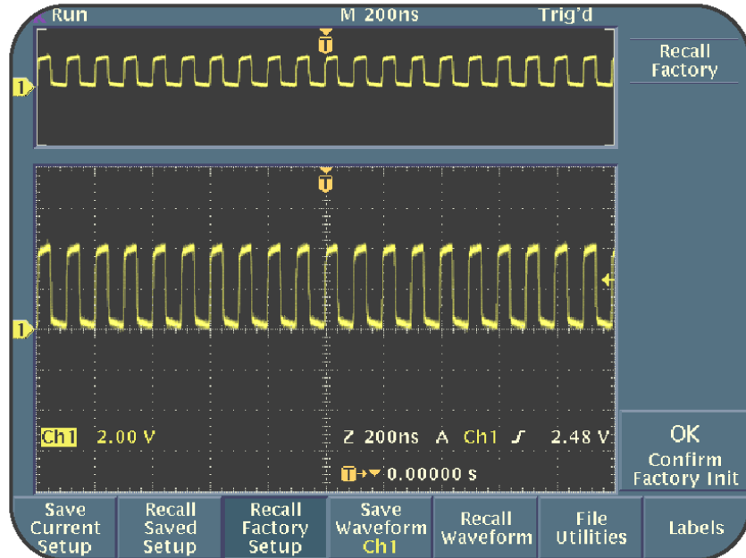
Figure 3.3: Zoom mode waveform display
