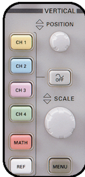
Figure 1.3: TDS3000 VERTICAL section controls
