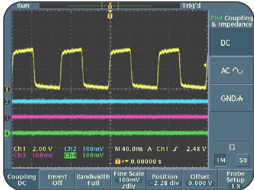
Figure 2.4: 4 Channel display
