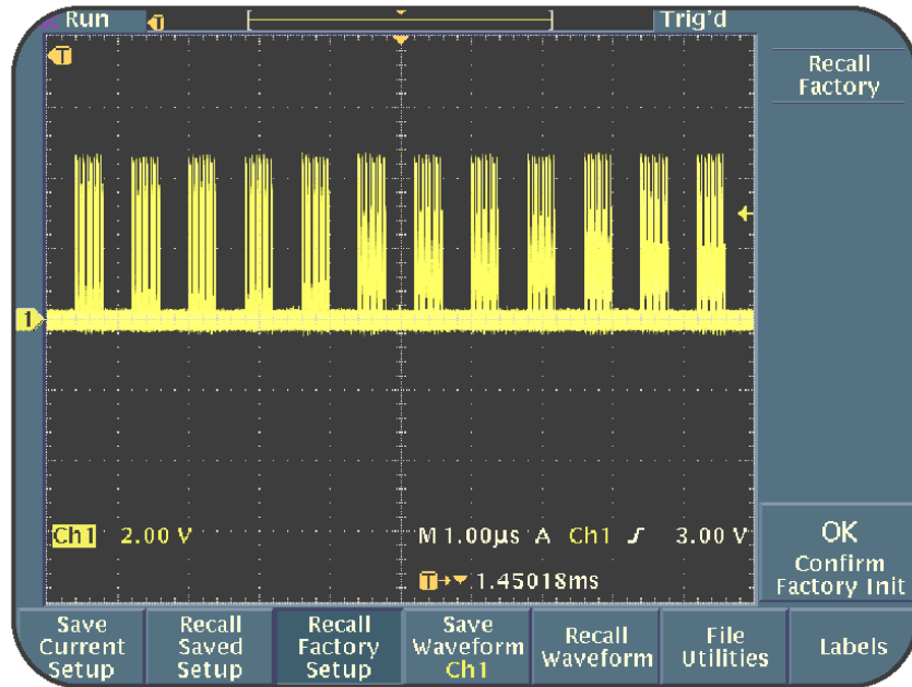
Figure 3.6: Unstable overlapping waveforms
