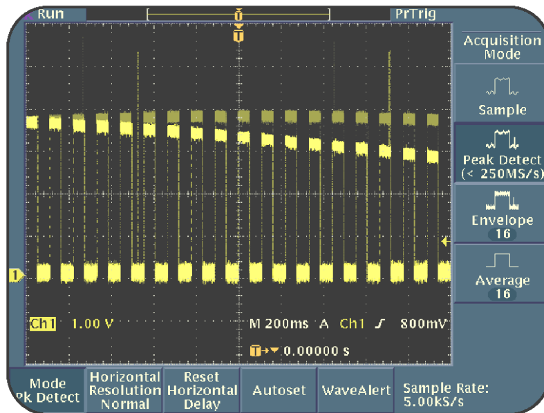
Figure 5.4: Noisy variable amplitude signal with glitches, captured with Peak Detect mode in an intensity graded display
