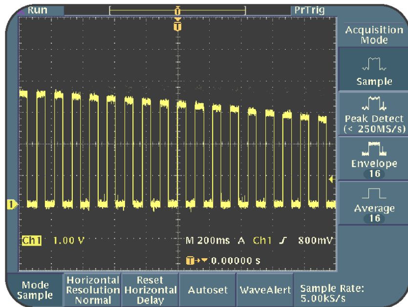
Figure 5.2: Noisy variable amplitude signal
