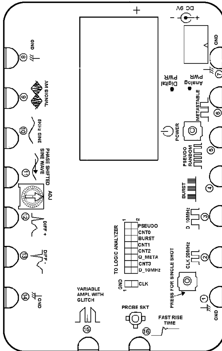
Figure 1.18: The Training 1 signal board
