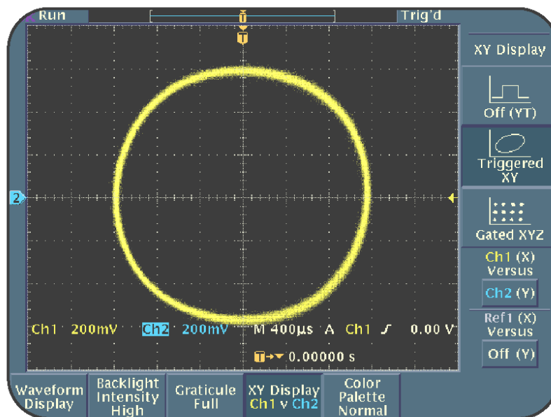
Figure 6.13: Phase relationship between two synchronous sine waves in the XY display format
