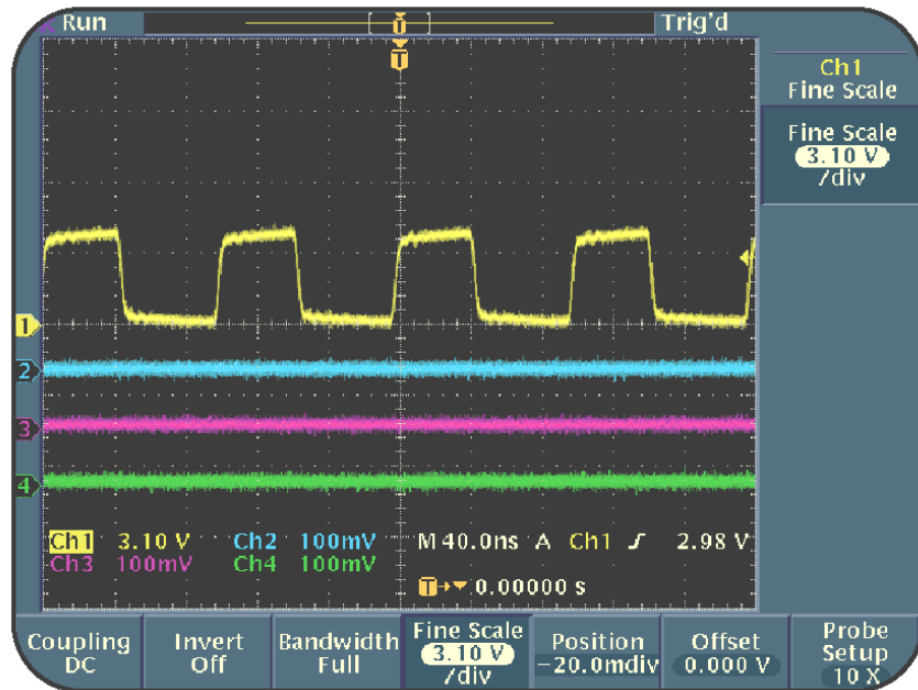
Figure 2.5: Modified input coupling
