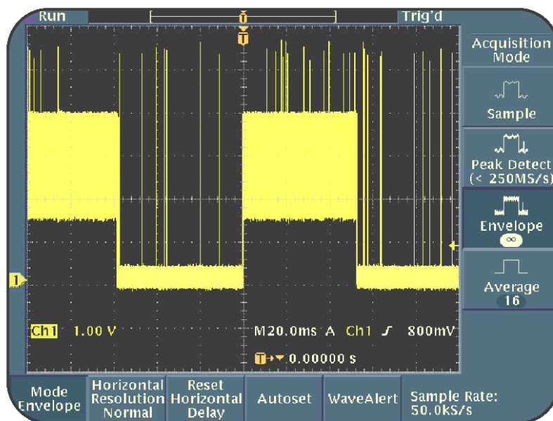
Figure 5.6: Accumulated peak-detected waveforms with the Envelope acquisition mode
