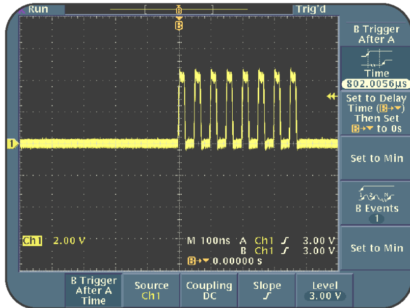
Figure 3.7: B TRIG enabled after a delay of about 800µs
