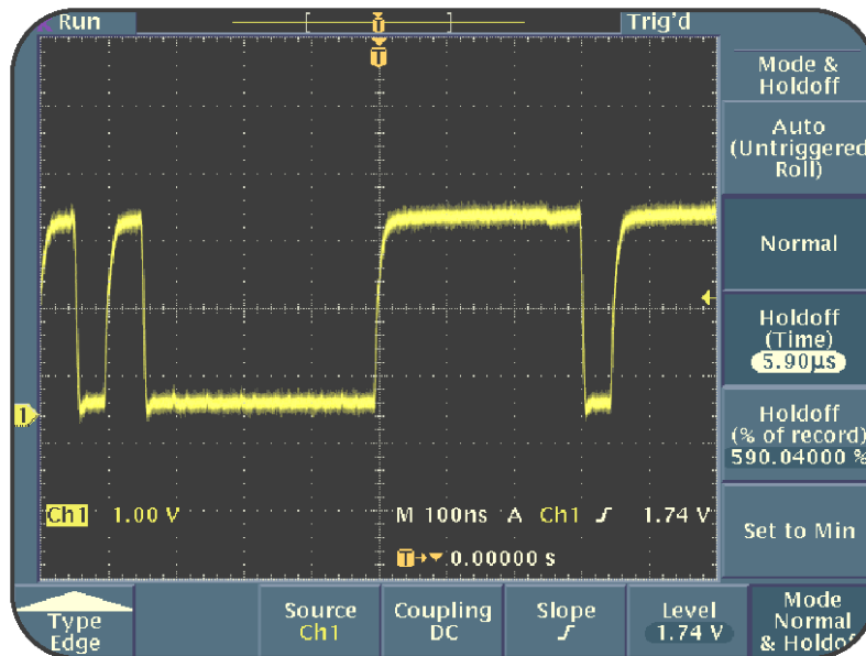
Figure 4.4: Triggering on complex repeating signals using trigger holdoff
