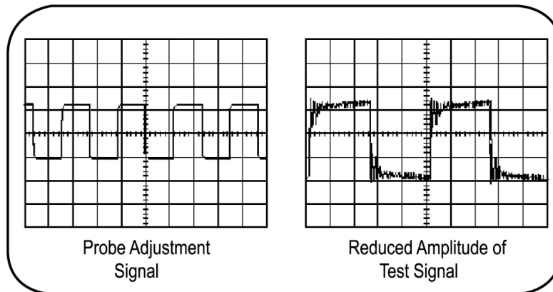
Figure 1.20: Undercompensated probe
