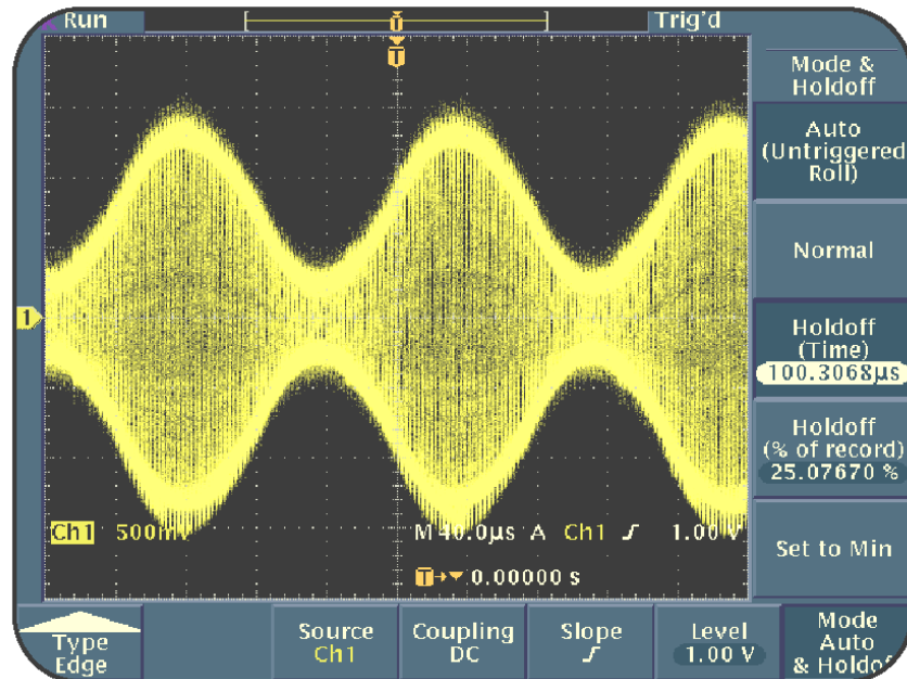
Figure 4.5: AM signal, with trigger holdoff
