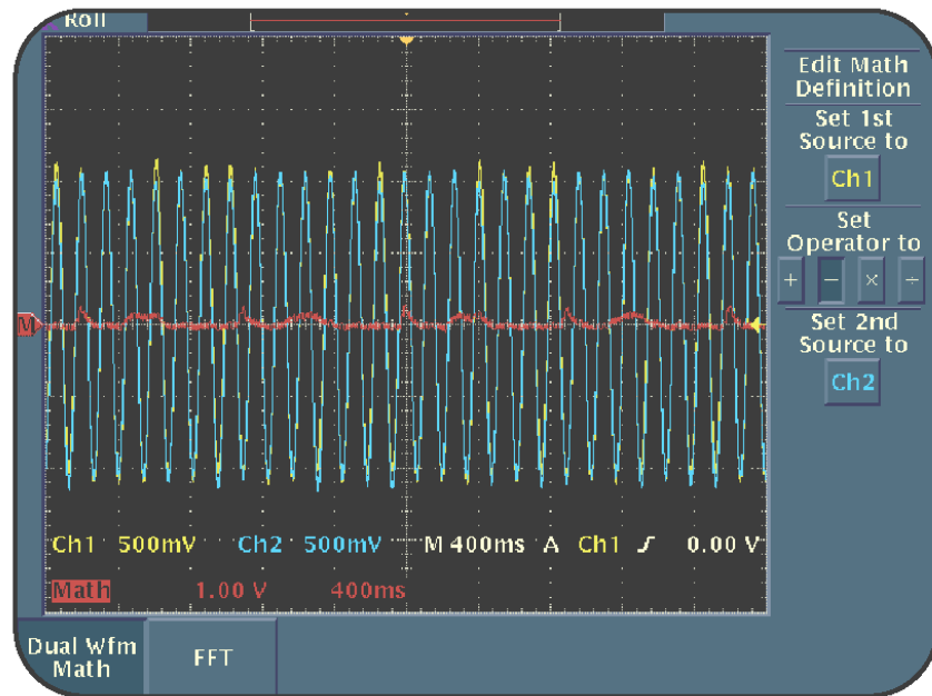
Figure 2.8: CH1-CH2
