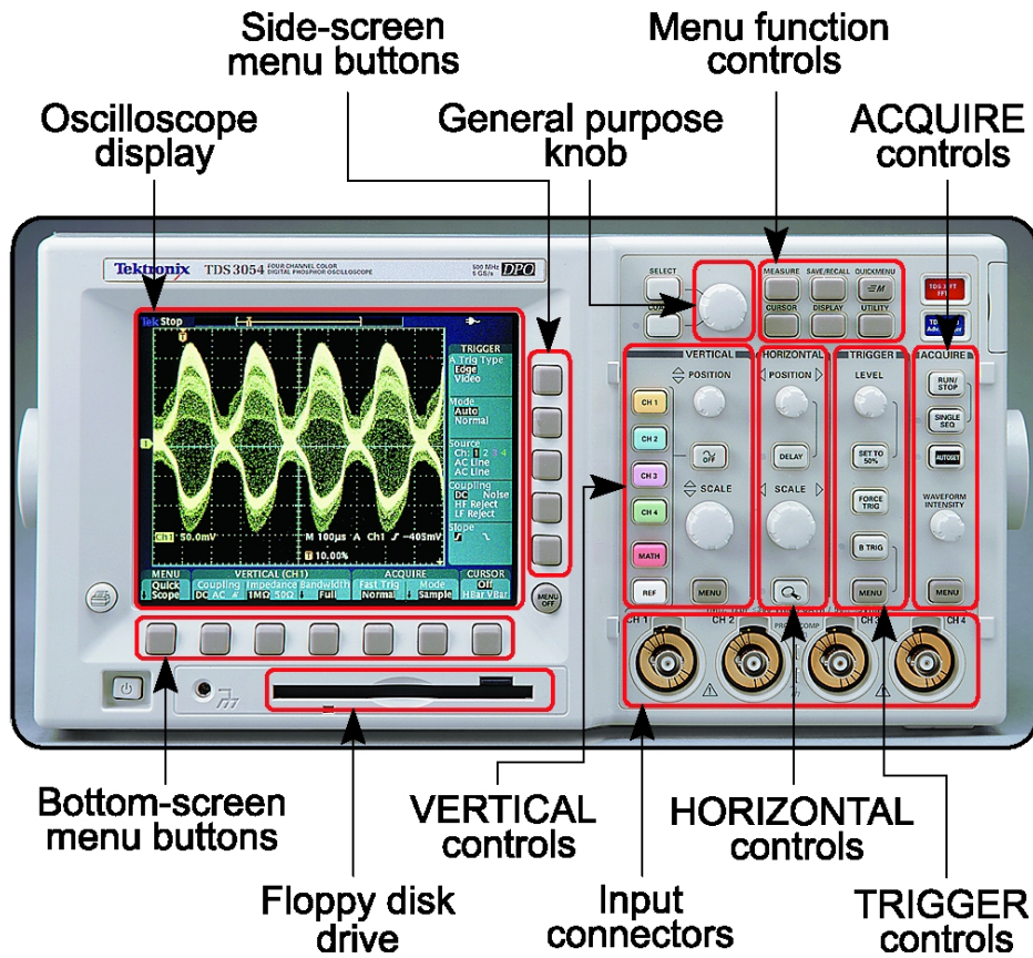
Figure 1.1: A TDS3054 digital phosphor oscilloscope
