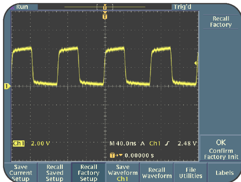
Figure 2.2: CLOCK signal
