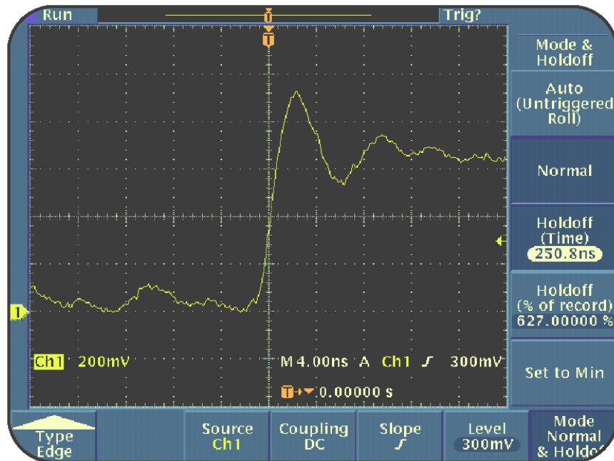
Figure 5.7: Step response waveform with ground lead
