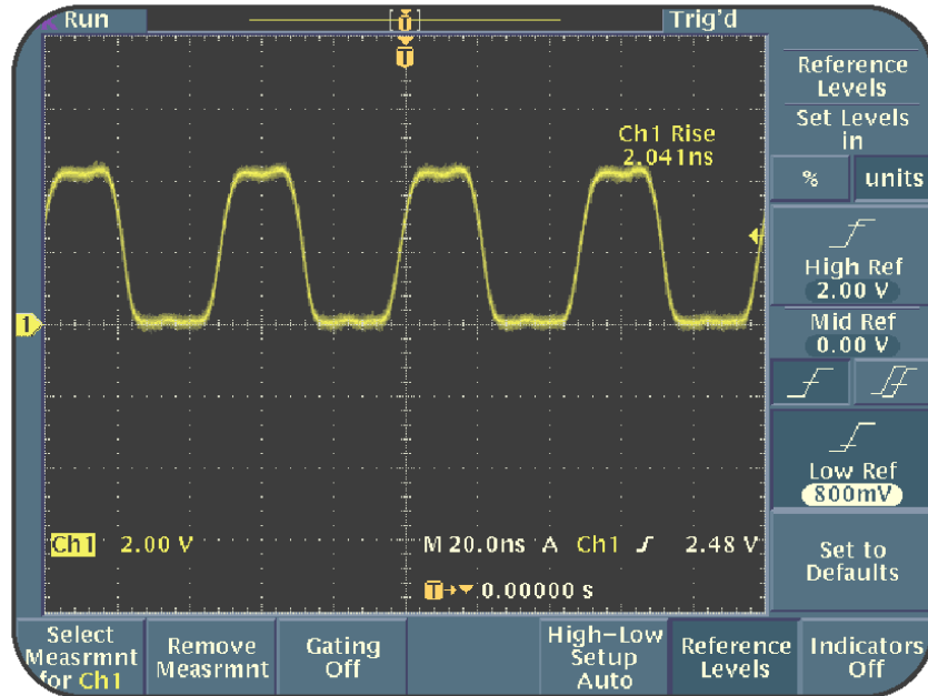
Figure 6.5: Verifying an incoming signal
