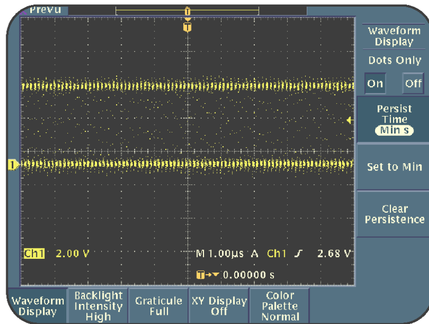
Figure 6.12: Clock signal with Dots Only On
