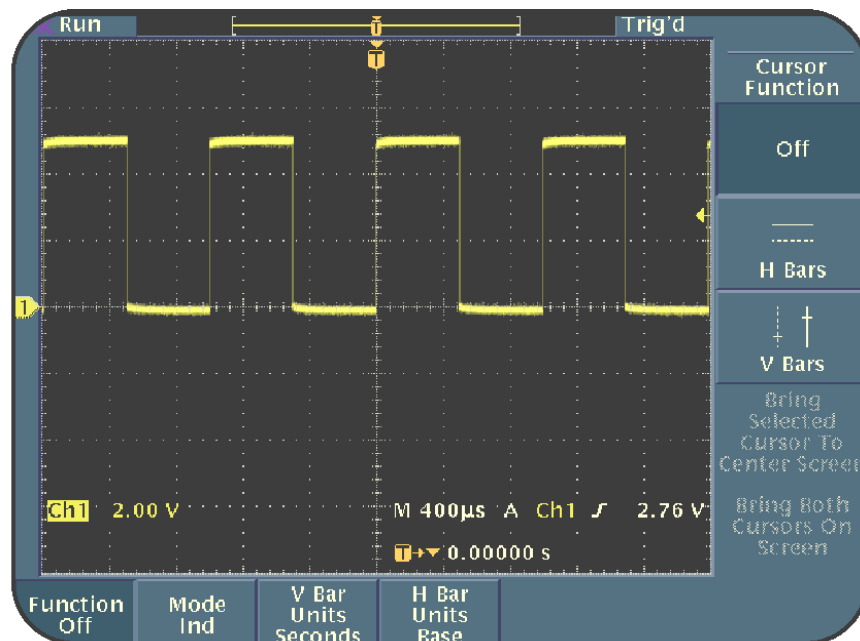
Figure 1.15: CURSOR menu
