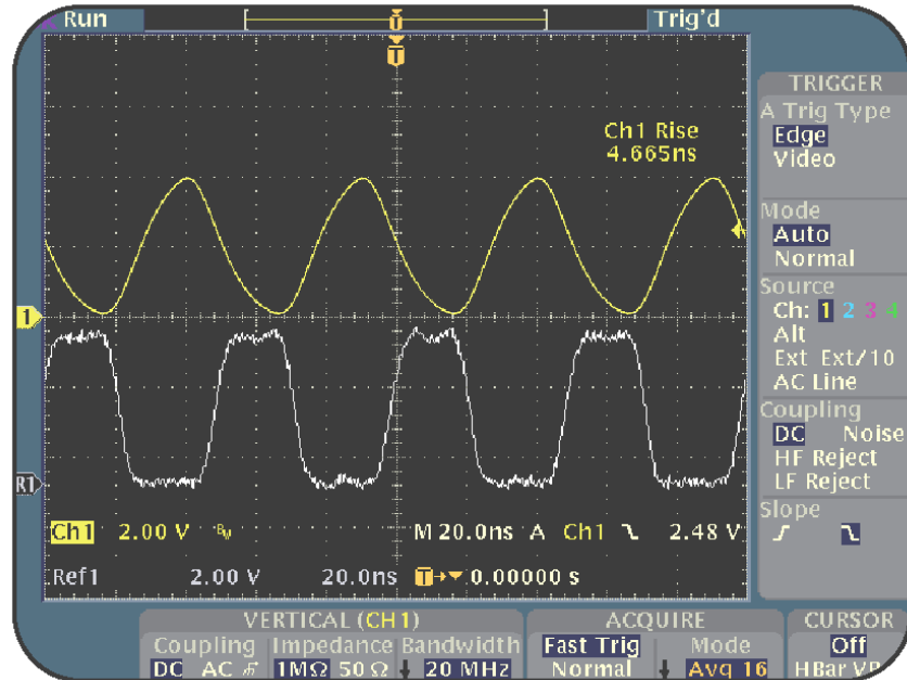
Figure 6.8: QUICKMENU display
