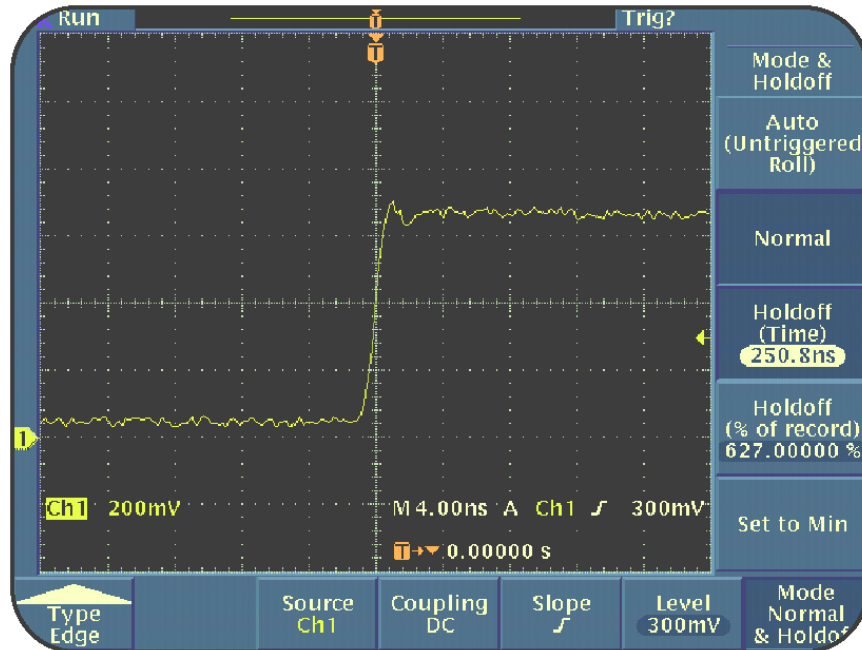
Figure 5.8: Step response waveform, without ground lead and probe tip extension
