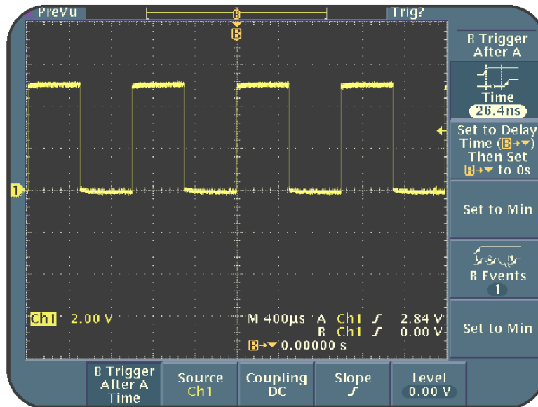
Figure 1.8: Menu-based controls for the B TRIG button
