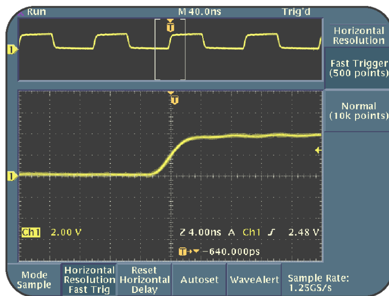
Figure 3.5: Magnified display with Fast Trigger (500 points) mode
