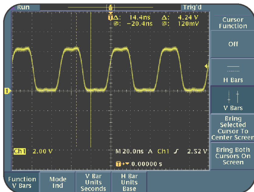
Figure 6.9: Cursors V Bar measurement
