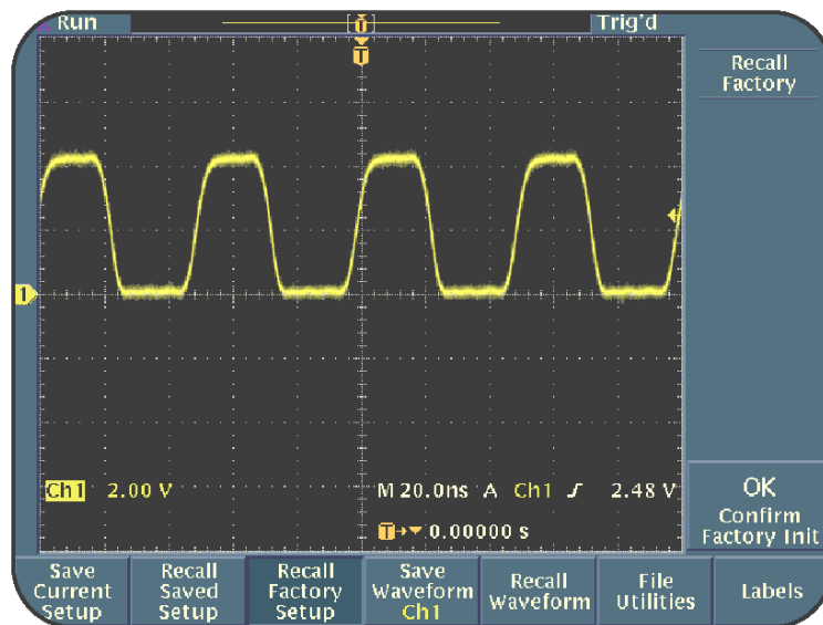
Figure 6.2: 20 MHz CLOCK signal
