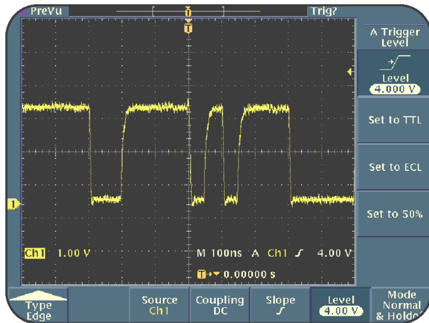
Figure 4.3:Edge triggering
