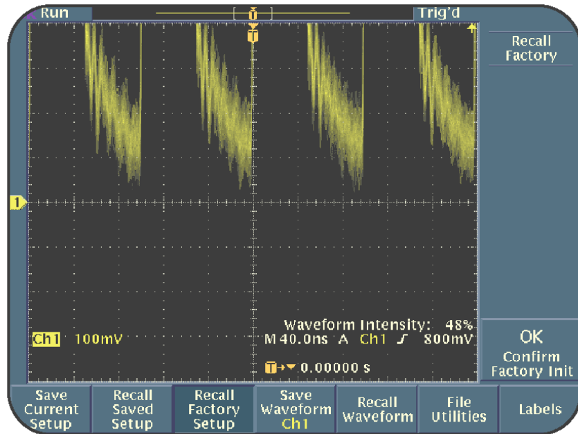
Figure 2.6: Vertically expanded waveform around the center graticule line
