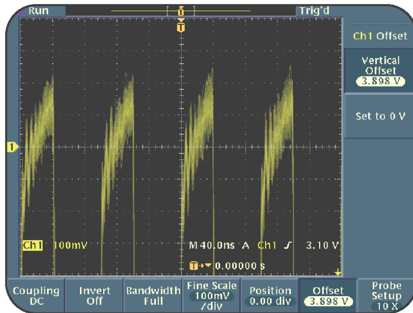
Figure 2.7: Changed vertical waveform expansion reference with respect to a waveform
