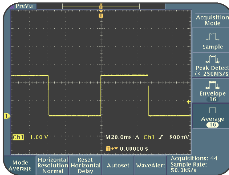
Figure 5.5: Reduced signal noise with the Average acquisition mode
