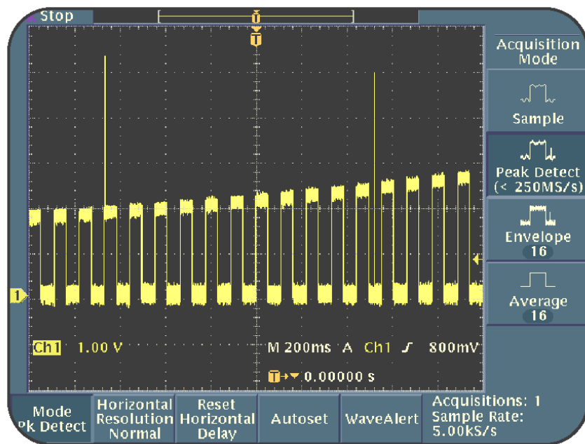
Figure 5.3: Noisy variable amplitude signal with glitches, captured with Peak Detect in SINGLE SEQ mode
