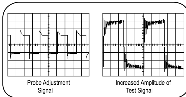
Figure 1.21: Overcompensated probe
