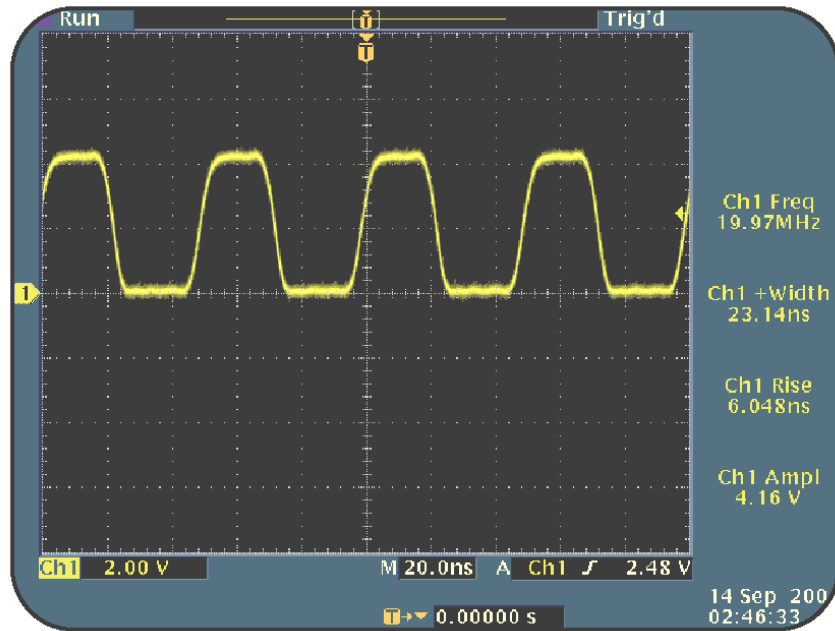
Figure 6.3: Automatic measurements
