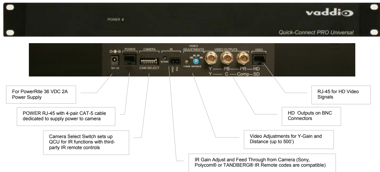
Figure 2: Quick-Connect PRO (QCP) Universal interface front panel and rear panel images with functional callouts.
