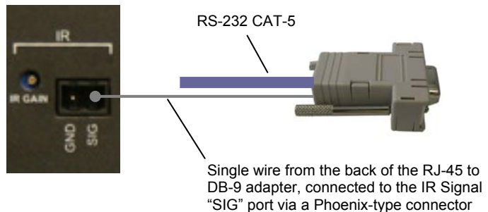
Figure 5: Required wiring configuration for IR Forwarding from the camera IR port to codec. Note: There is no IR port on the front of the HDX 8006 codec. The IR receiver on the codec is imbedded in the EagleEye 1080 HD camera. NOTE: Only the Camera 1 port on the HDX series codecs supports IR forwarding.
