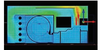
Unique LCD panel cooling system
