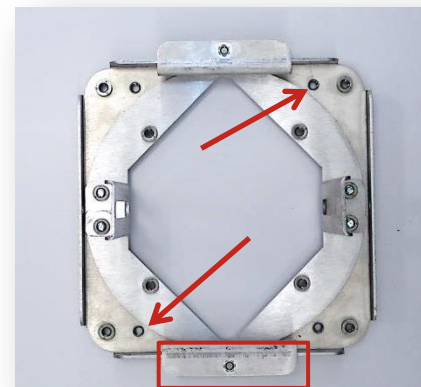
Rail clamp
