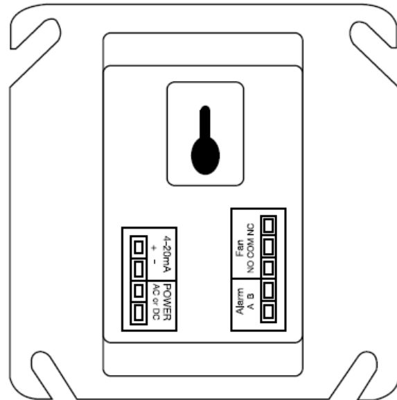
GD-3000 rear view with Modular Connectors
