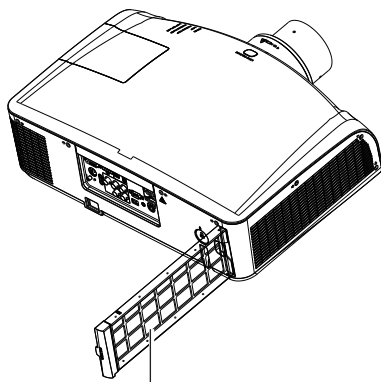
Air filter
