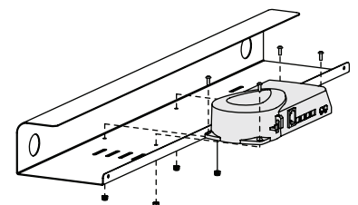
Attaching the Control Box to the Cable Tray of a shallow 48" wide table.
