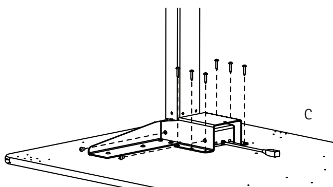
1" Btn-Hd Screw 325-5580-00
