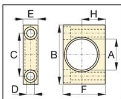
Foot Mounting Mounts onto cylinder collar. Mounting screws not included.
