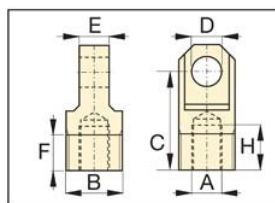
Clevis Eye Threads onto plunger or into cylinder base
