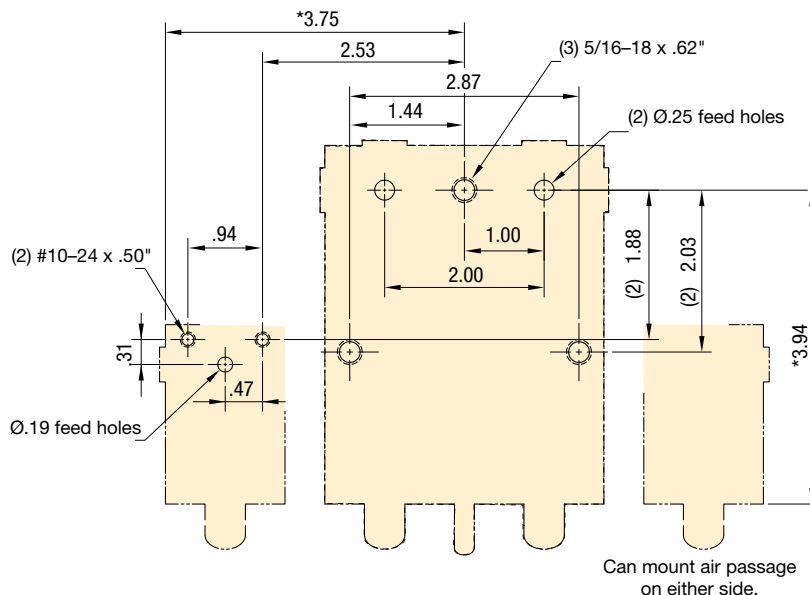
MCR-21 with MCRA-11 Receiver with air passage and without P.O. check – Mtg. hole pattern
