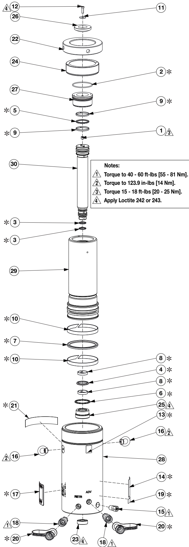
Figure 1, Exploded View - Model HCRL 502-506
