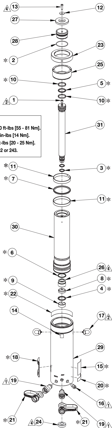
Figure 2, Exploded View - Model HCRL 508-5012
