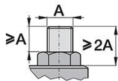
Minimum Stud Protrusion
