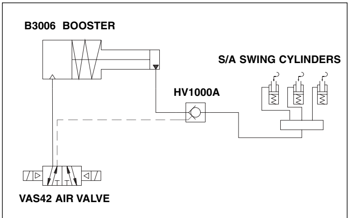
Figure 1. Example Circuit
