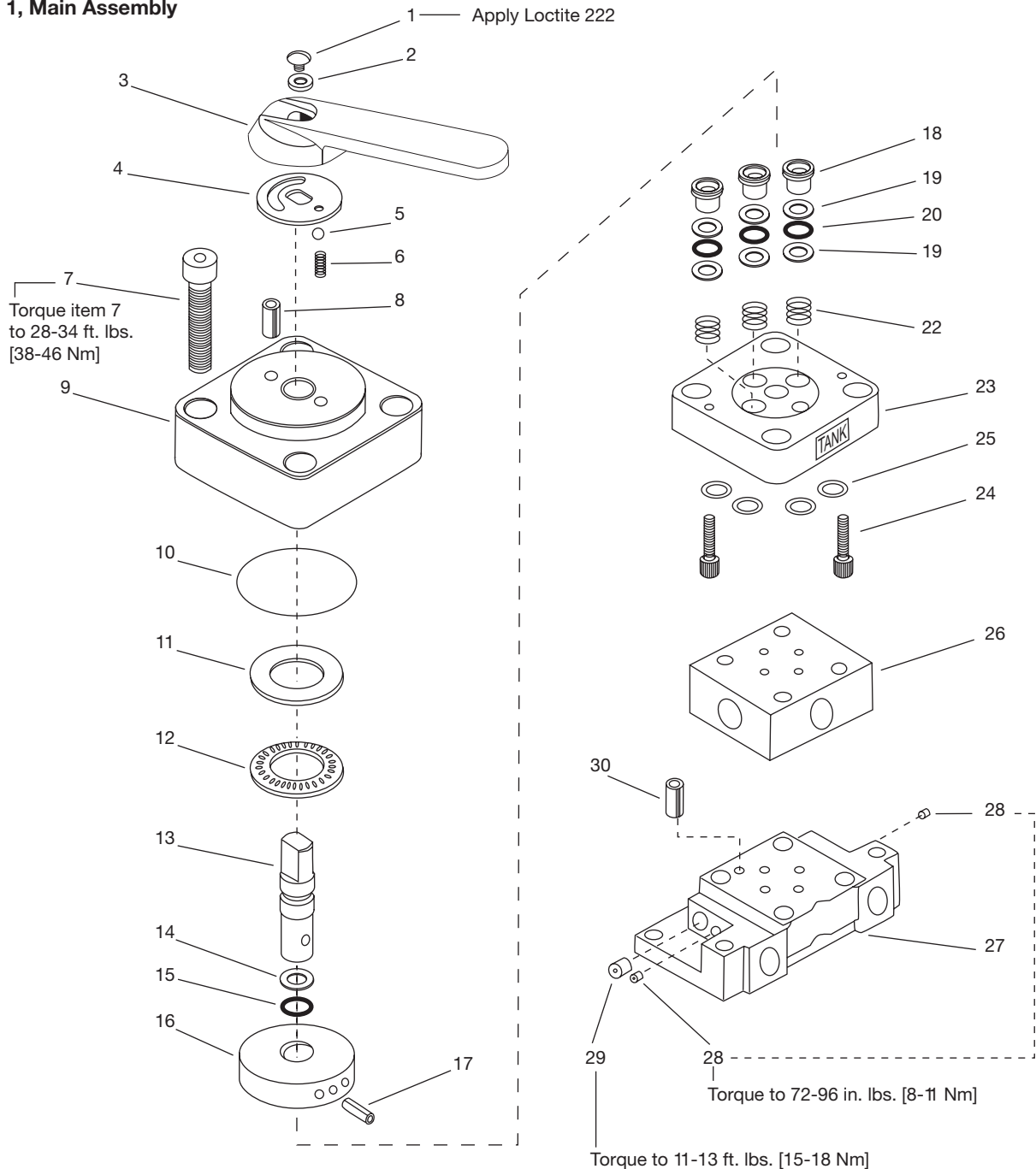
Figure 1, Main Assembly
