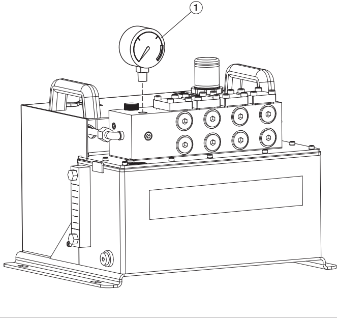
Figure 2 - Manifold / Valve Station
