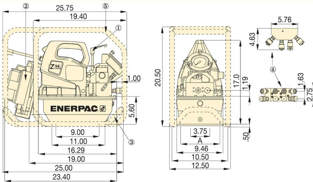
ZU4-Series Torque Wrench Pumps
